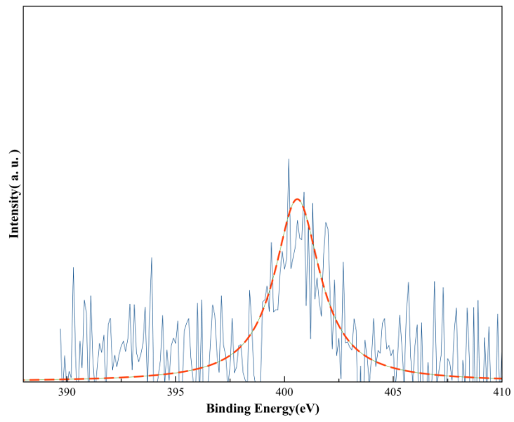
N 1s
