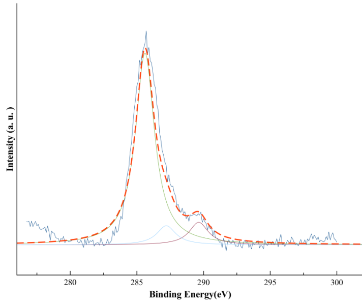
C 1s
