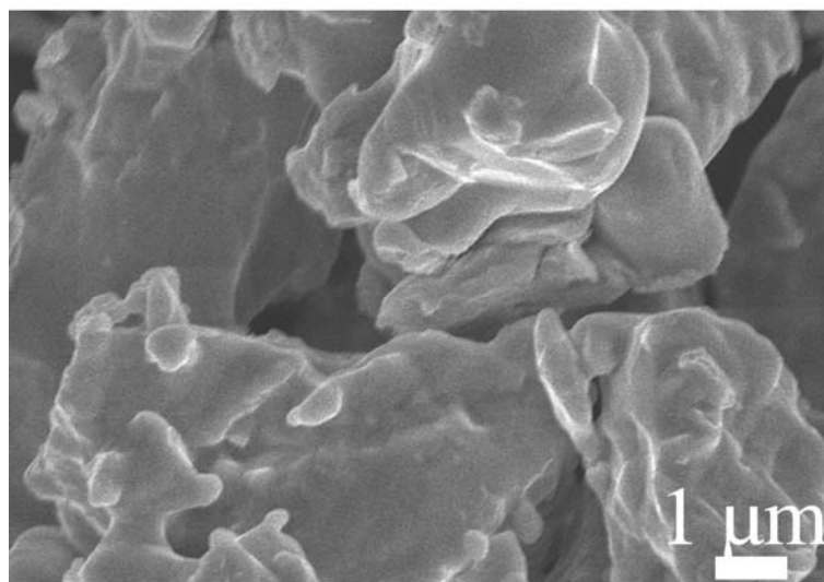
Figure S1. FE-SEM image of the Ti powders.
