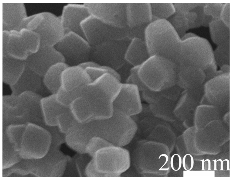
Figure S2. FE-SEM image of the flower-like TiO 2 nanostructures after heating at 600 °C for 2 h.
