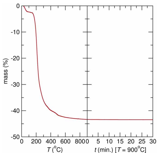
Figure 1S: TGA curve of the copolymer-templated mesoporous silica containing YAG:Ce nanoparticles, in air.
