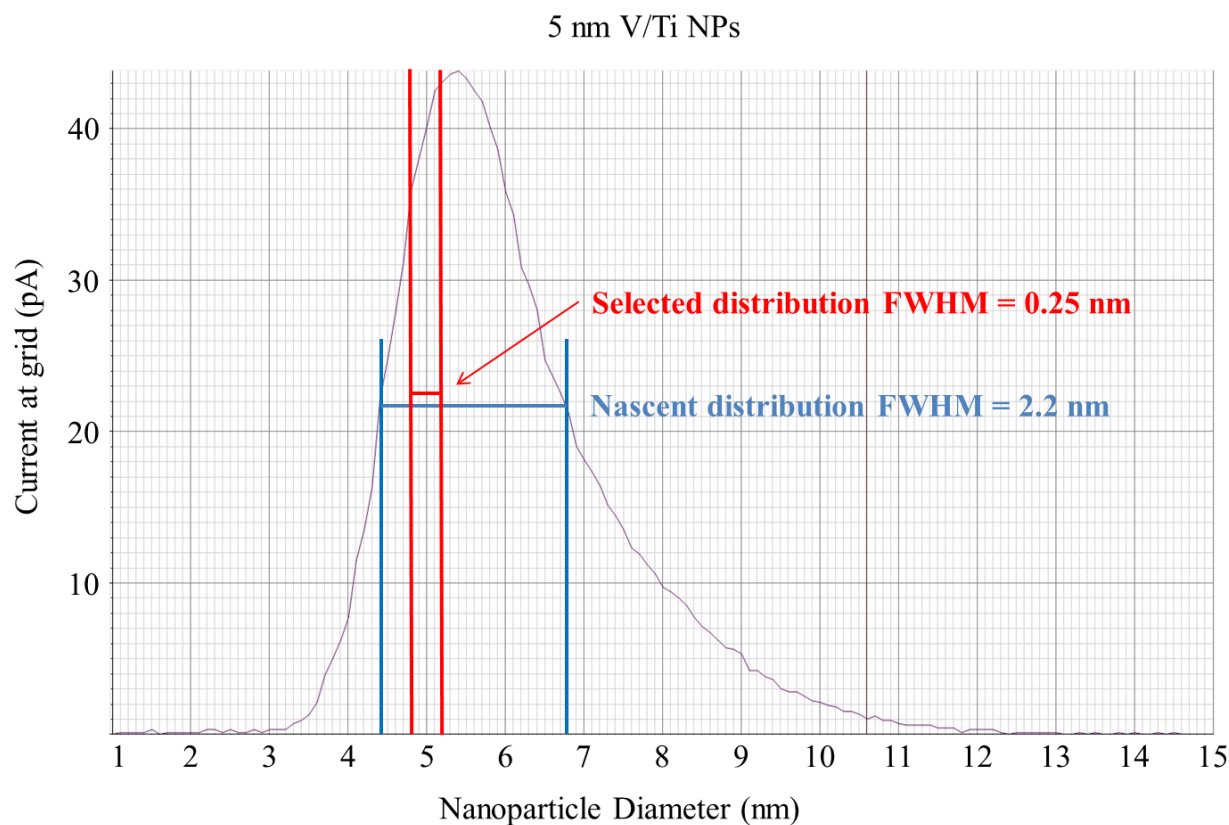
Figure S1. A representative spectrum of 5 nm V/Ti alloy nanoparticles obtained using the MesoQ mass filter. Note the substantially wider distribution of sizes in the nascent cluster distribution compared to the distribution selected by the mass filter.
