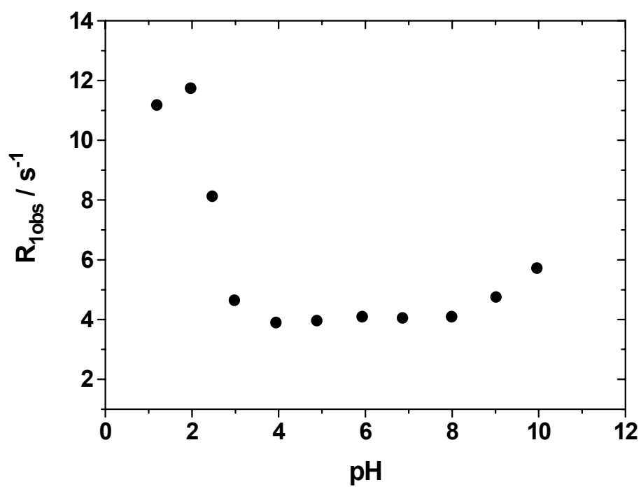
Figure S1 pH-dependence of relaxation rate (Gd-1, 20 MHz, 298K)
