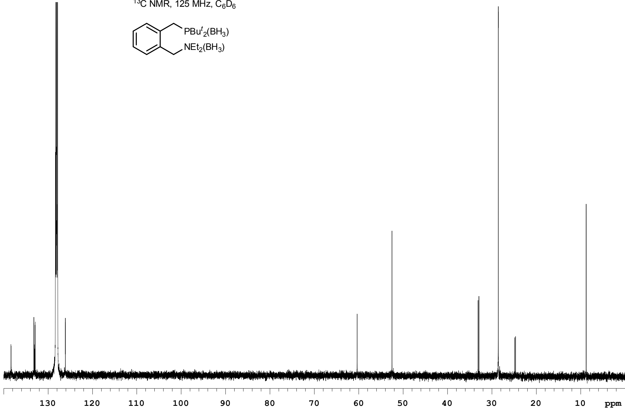
Compound 11c ^{13}\text{C} NMR, 125 MHz, \text{C}_6\text{D}_6
