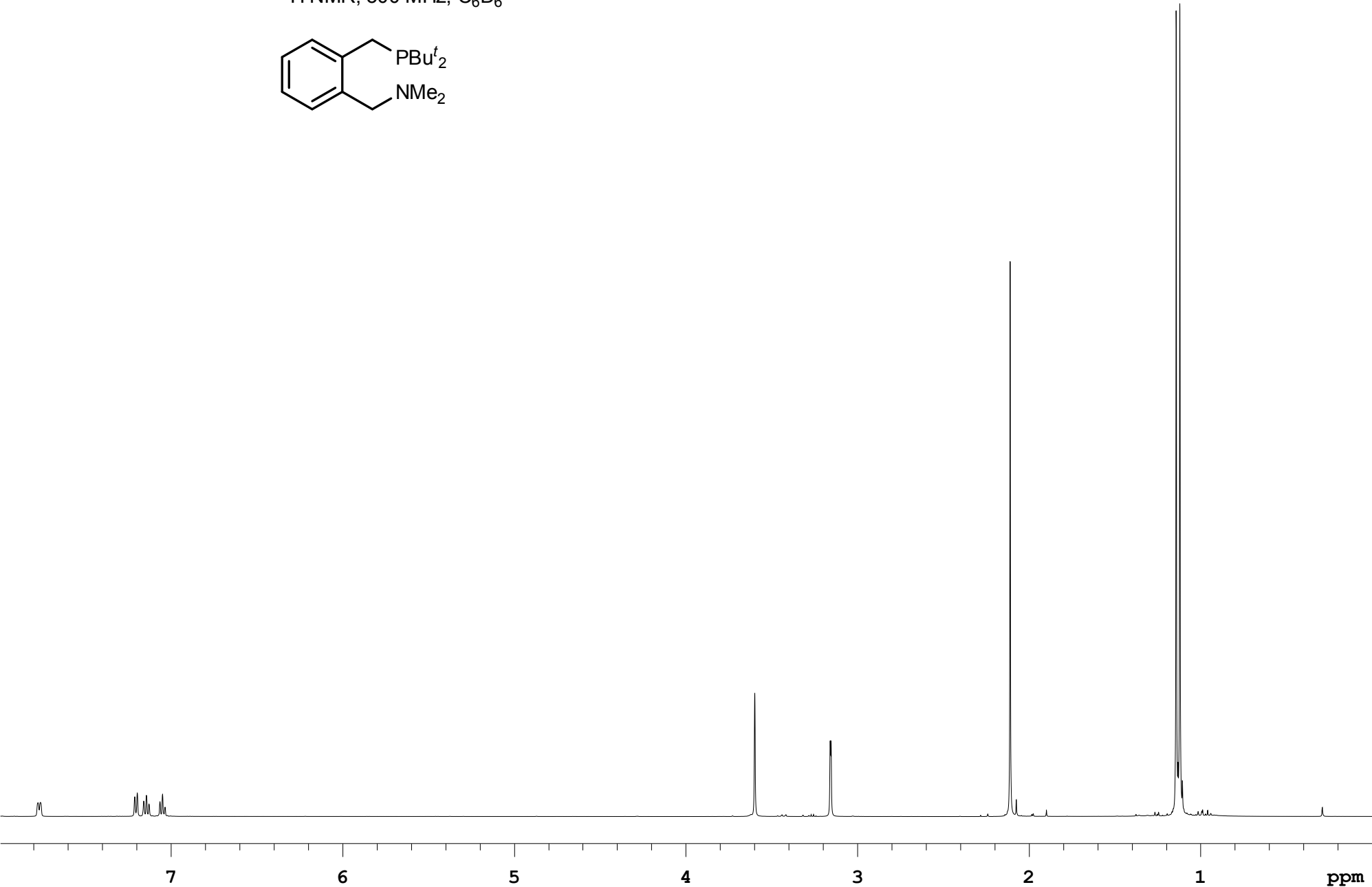
Compound 12a 1 H NMR, 500 MHz, C 6 D 6
