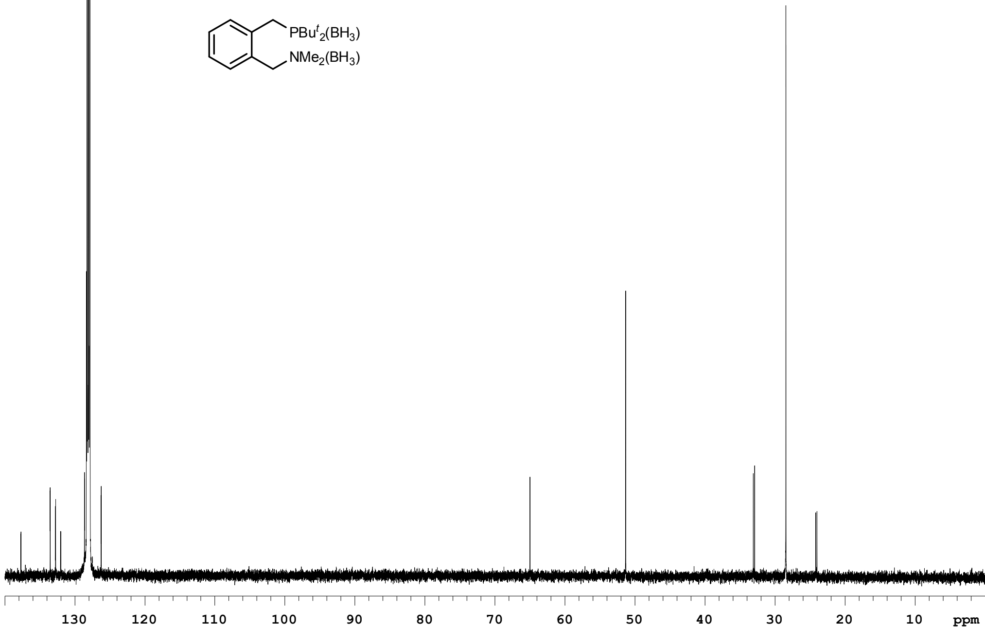
Compound 11a 13 C NMR, 125 MHz, C 6 D 6
