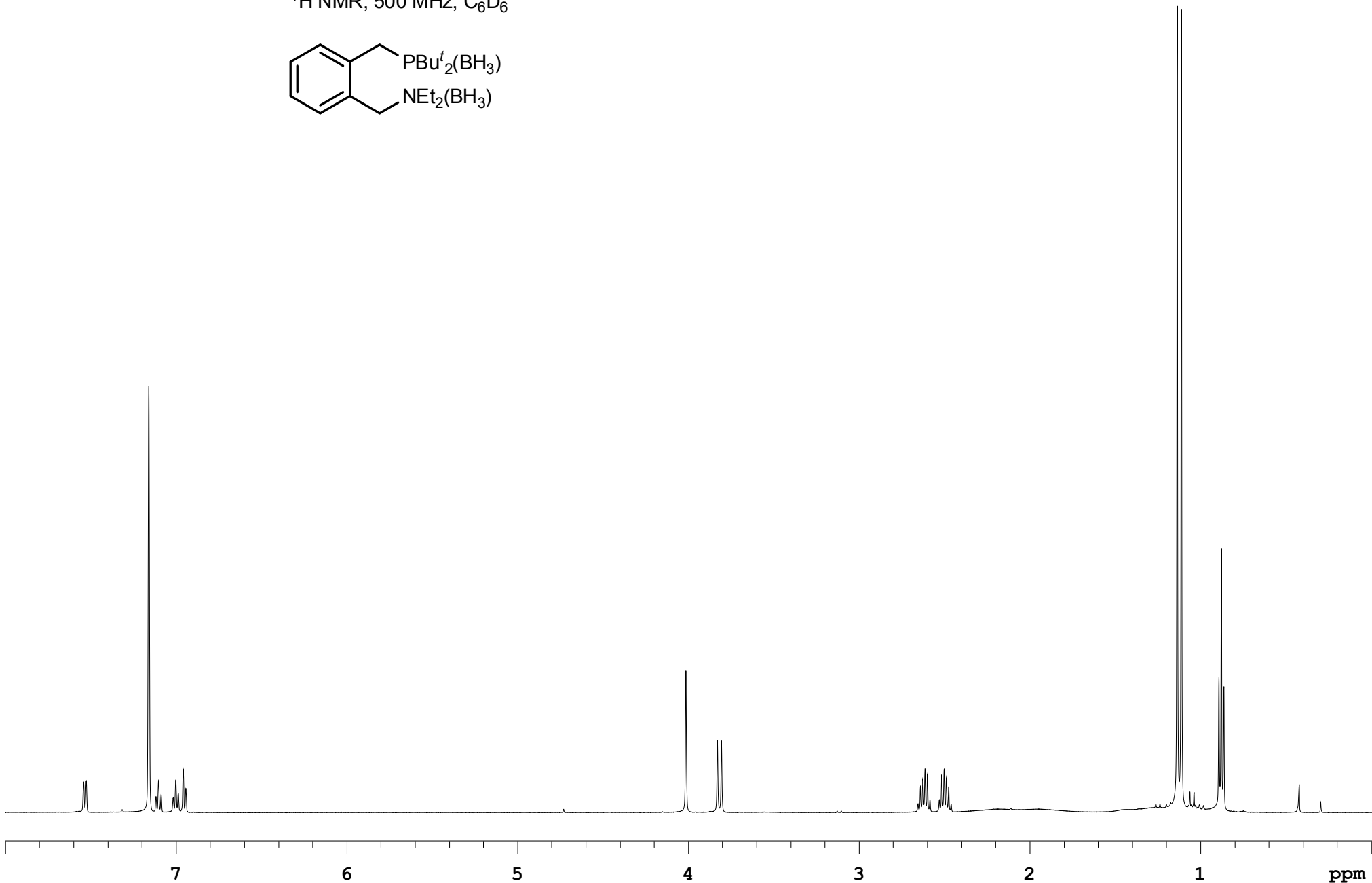
Compound 11c 1 H NMR, 500 MHz, C 6 D 6
