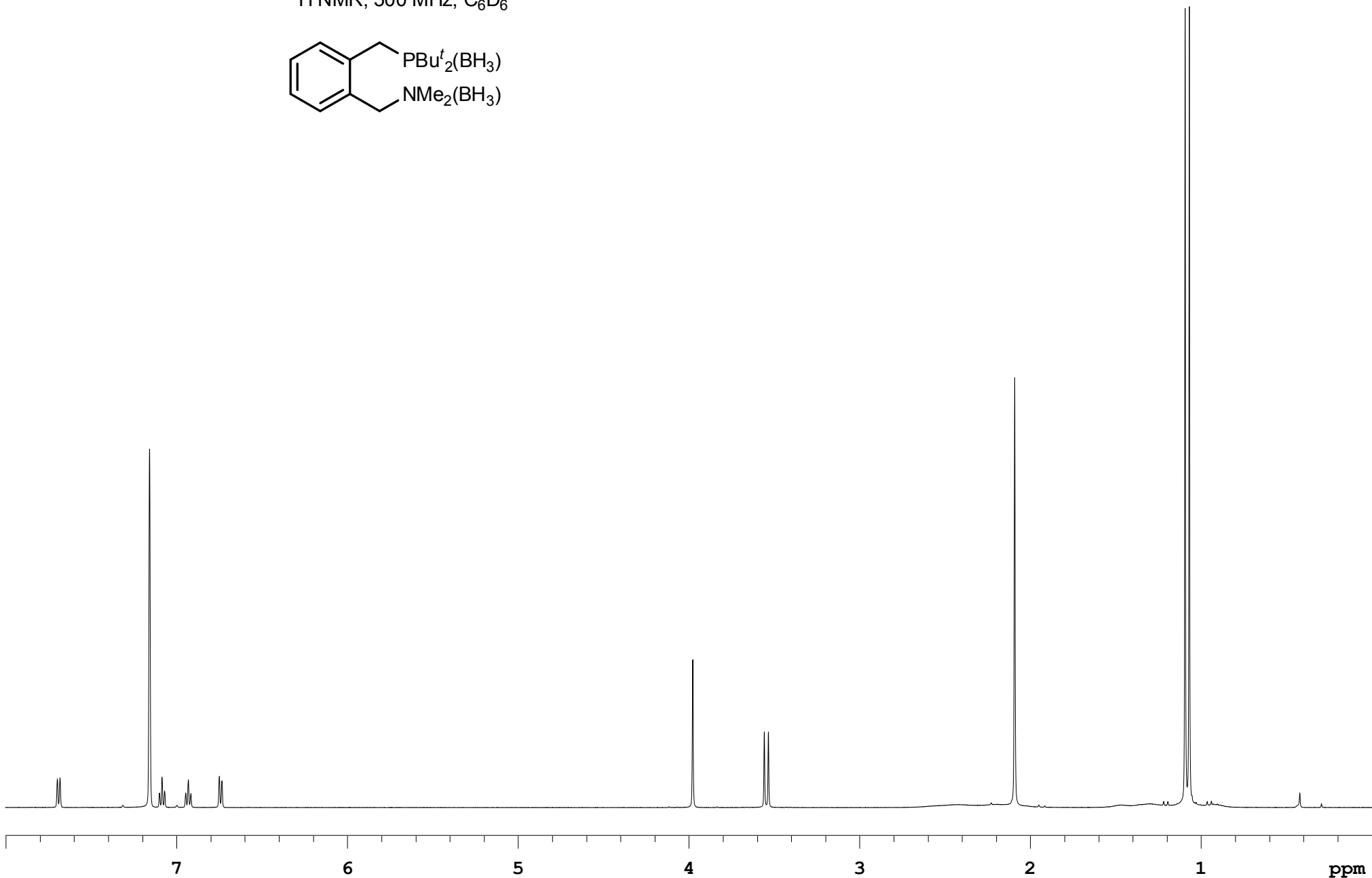
Compound 11a 1 H NMR, 500 MHz, C 6 D 6
