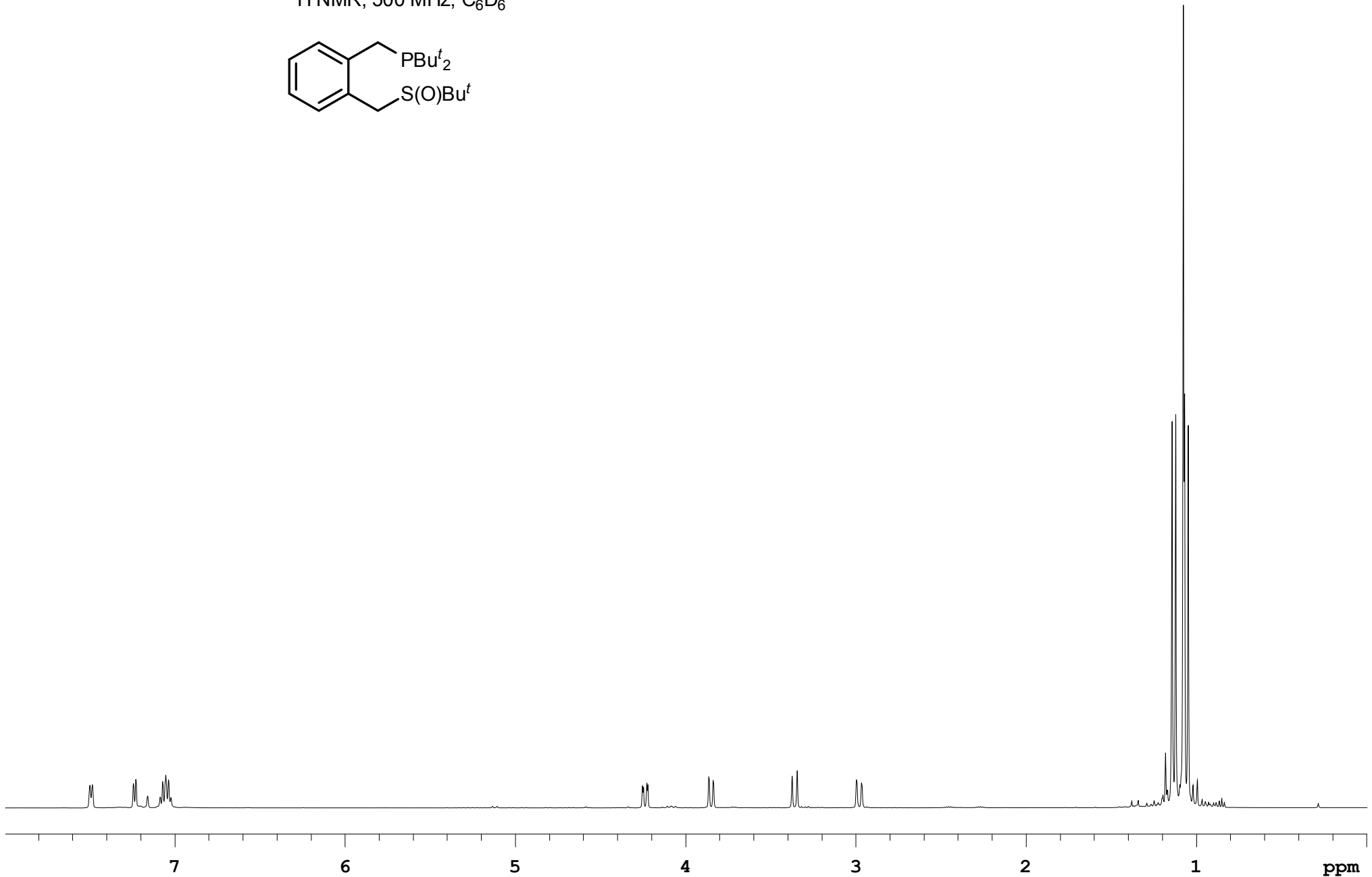
Compound 10 ^1\text{H} NMR, 500 MHz, \text{C}_6\text{D}_6
