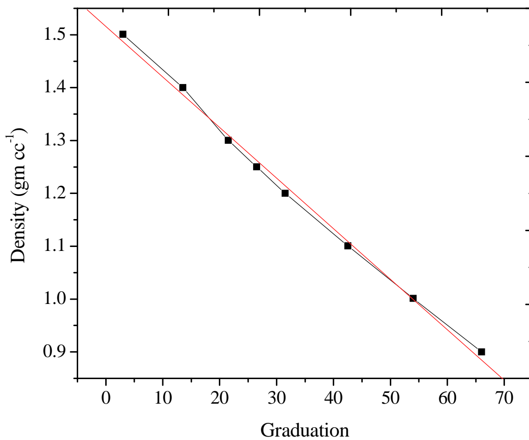
Fig. S2. Calibration curve for the density gradient column
