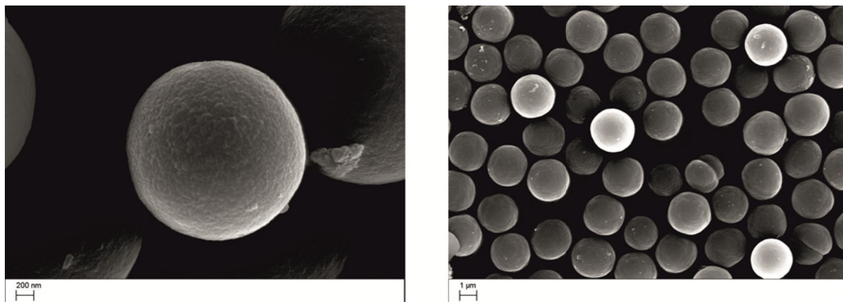
Figure S4: Scanning electron microscopy (SEM) images of microspheres synthesized via distillation precipitation polymerization with addition of 8.6 wt% PBN (microsphere 2), showing monodisperse microspheres with a smooth surface.
