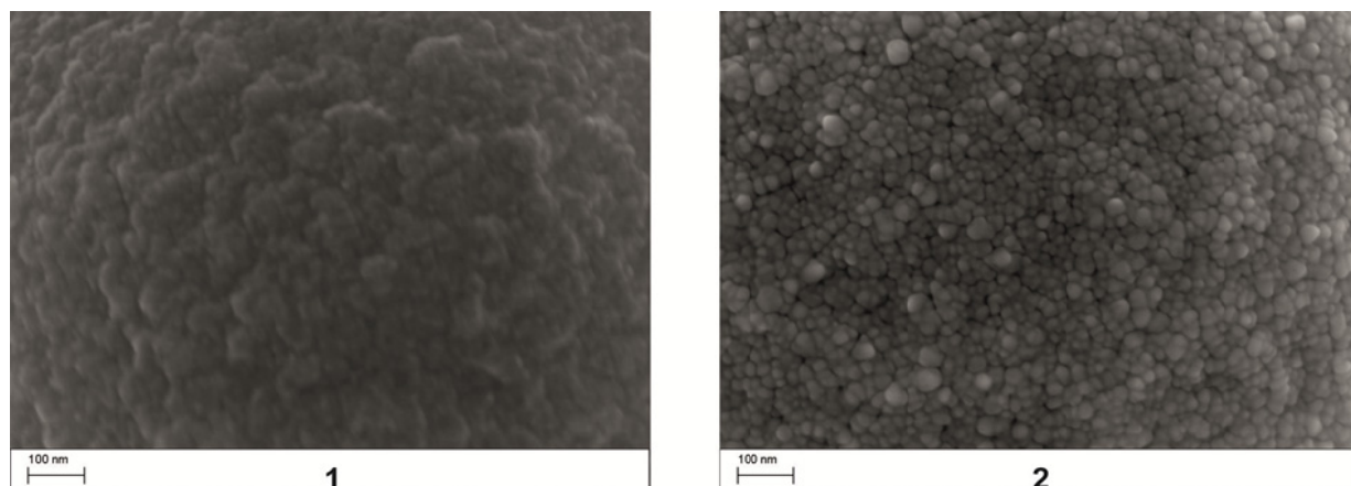
Figure S5: Close-up view of the microsphere surfaces before (1) and after (2) the nitroxide mediated polymerization. The smooth surface of the original microsphere becomes substantially rougher. The small exaltations are an indication for formed polymeric ‘loops’.
