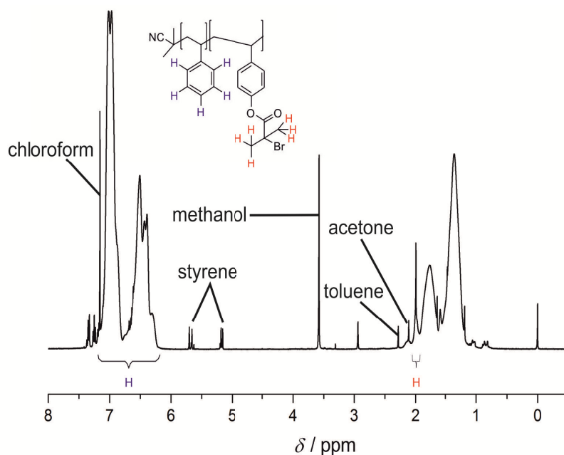
Figure S2: 1 H NMR spectrum of a copolymer containing styrene and VBMP. Protons of different organic small molecules present during the synthesis are also visible in the spectrum.
