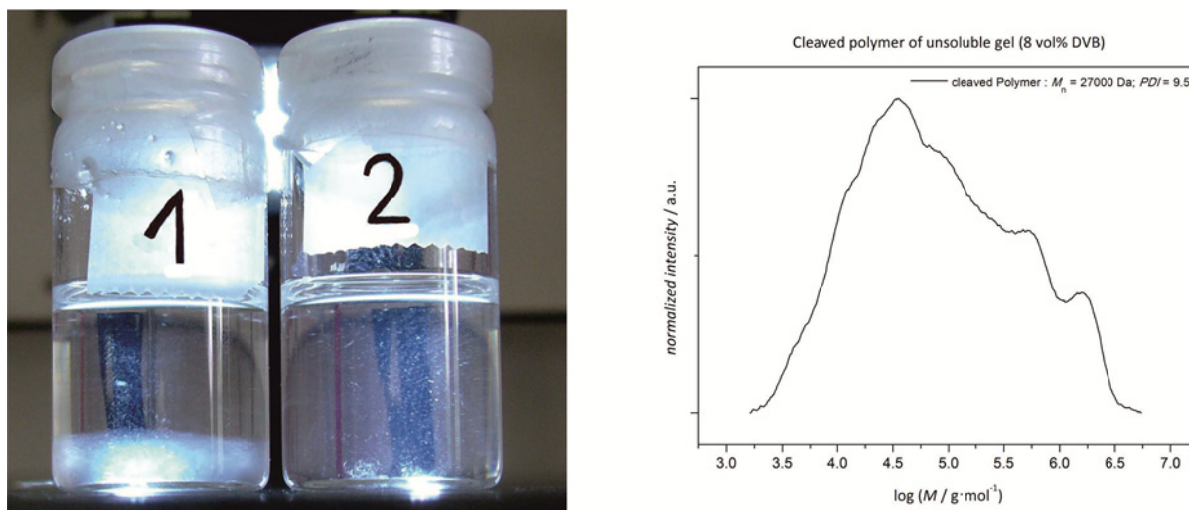
Figure S1: Photographic comparison of THF solubility of 8 vol% DVB gel before (1) and after (2) cleavage (left) and SEC analysis of the cleaved product ( M_n = 27\,000\text{ g}\cdot\text{mol}^{-1} ; PDI = 9.5) (right).
