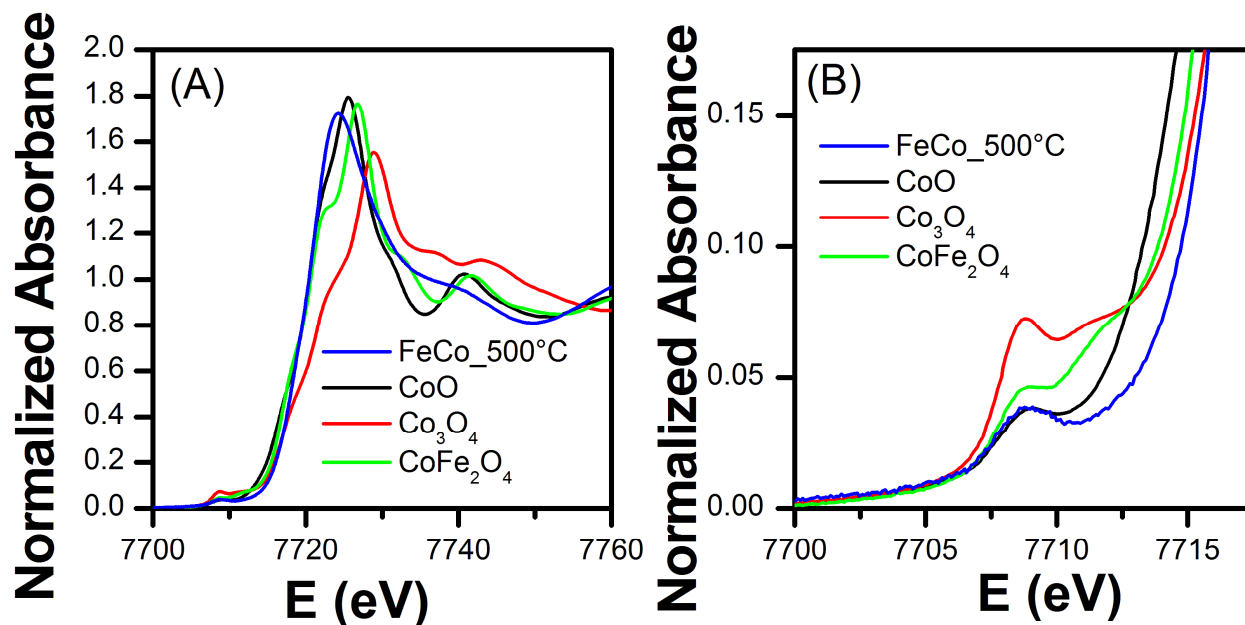
Figure 2. XANES spectra at the Co K-edge for FeCo_500°C and a series of Co oxides used as reference compounds (A) and details of the pre-edge peak (B).
