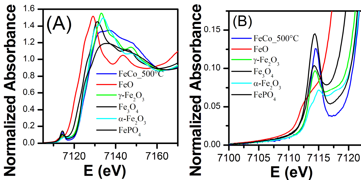
Figure 1. XANES spectra at the Fe K-edge for FeCo_500°C and a series of Fe oxides used as reference compounds (A) and details of the pre-edge peak (B).
