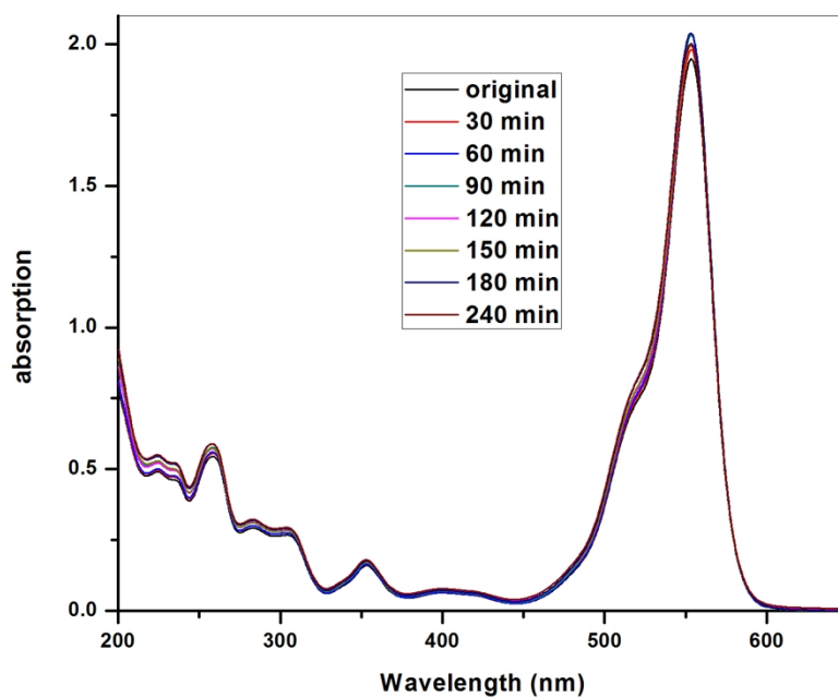
Fig. S2 UV-Vis. Spectral changes of RhB under visible light irradiation (without any catalyst).
