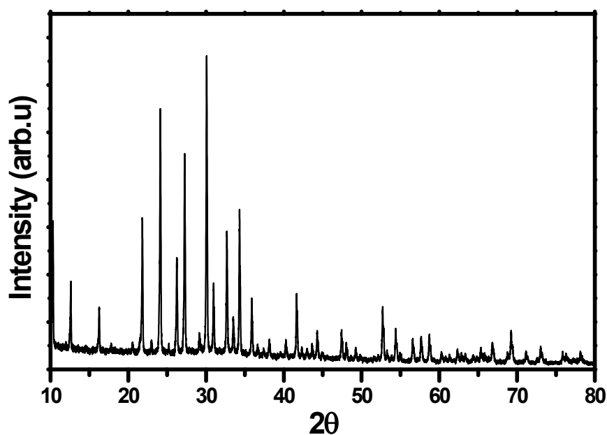
Fig. S1 PXRD of pure Zeolite-Y.
