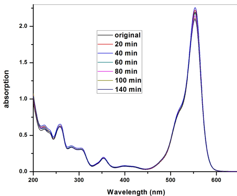
Fig.S3 UV-Vis. Spectral changes of RhB under UV light irradiation (without any catalyst).
