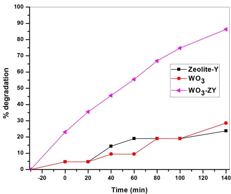
Fig. S5 % degradation of RhB under UV light irradiation by different catalyst.
