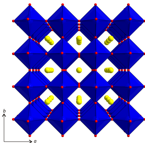
Polyhedral representation of \text{La}_{0.1}\text{Sr}_{0.9}\text{Co}_{1-x}\text{Nb}_x\text{O}_3 in the ab -plane (blue, Co(1) or Nb(1); yellow, Sr(1) or La(1); red, O).
