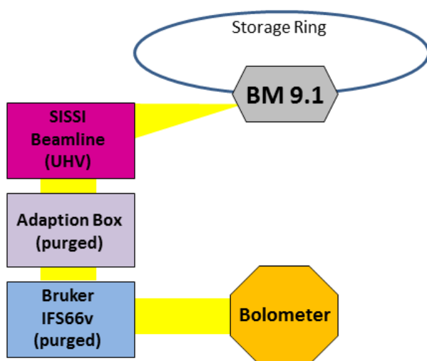
Figure S2. Schematic description of the SISSI beamline.
