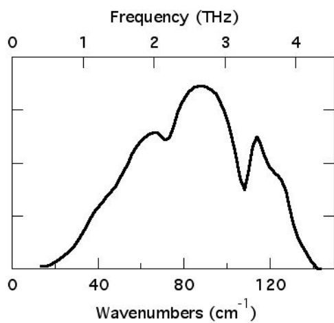
Figure S3. Spectrum of recorded THz radiation at the SISSI beamline with the described detector configuration.
