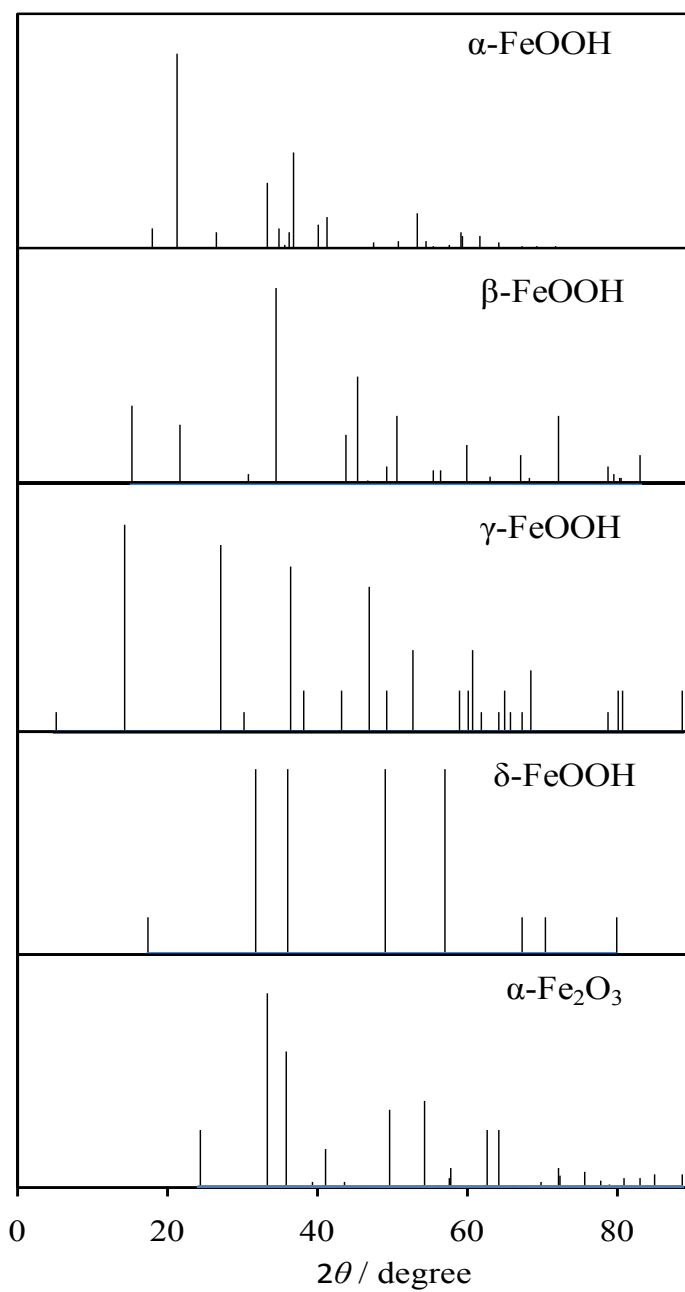
Fig. S1. The standard XRD patterns of four kinds of iron (oxy-hydr)oxide.
