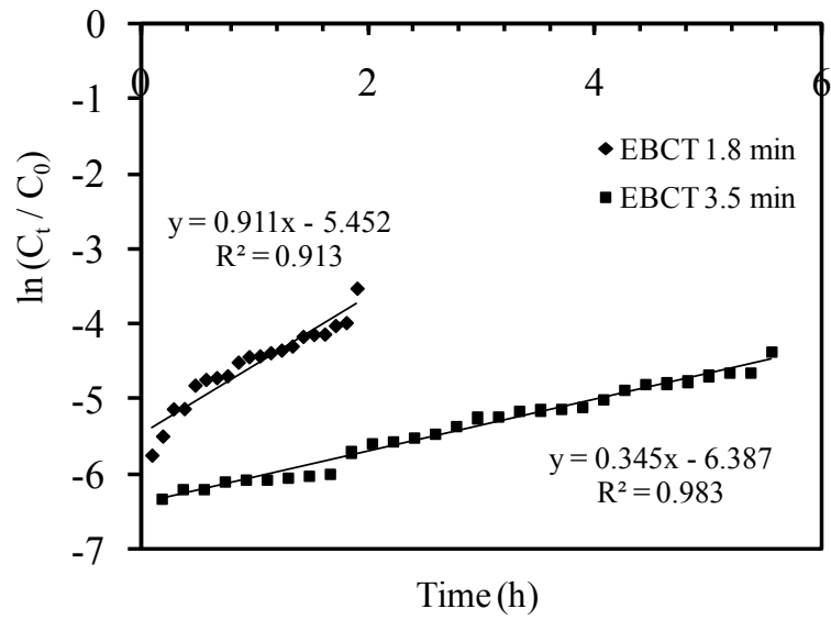
Fig. S2. Adams-Bohart model for the continuous adsorption of As(III).
