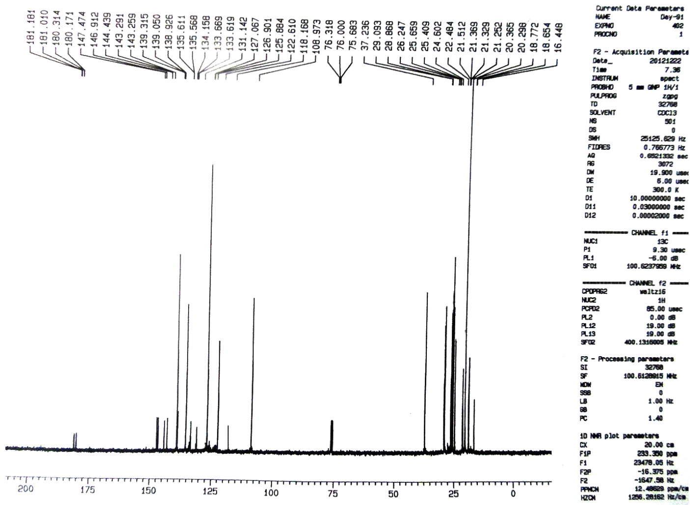
Supplementary 2.2. ^{13}\text{C} -NMR of Ortho-diacetate aethiopinine (2)
