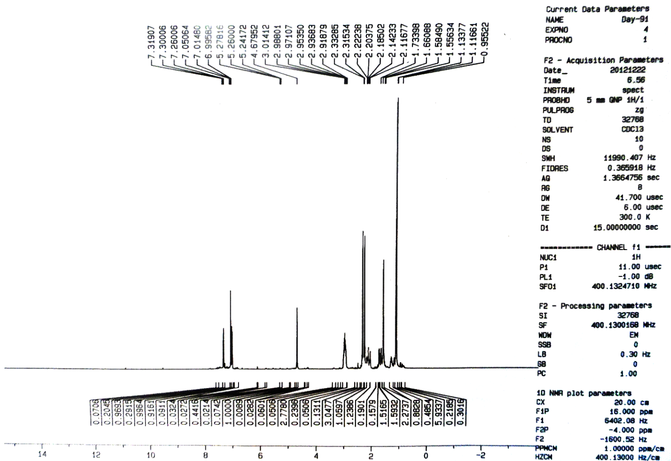
Supplementary 2.1. 1 H-NMR of Ortho-diacetate aethiopinone (2)
