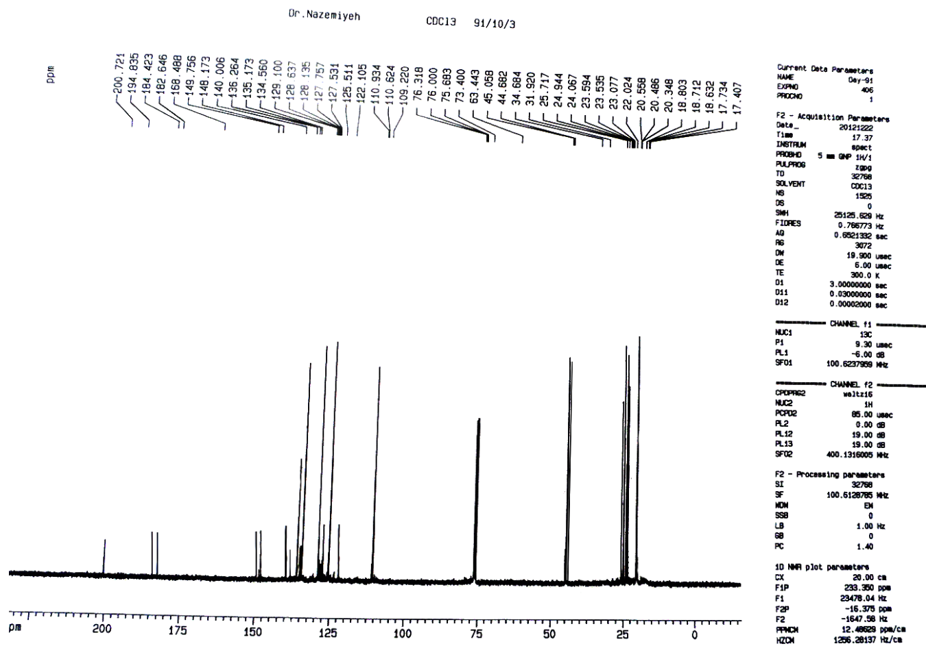
Supplementary 1.2. ^{13}\text{C} -NMR of Ketoethiopinone (1)
