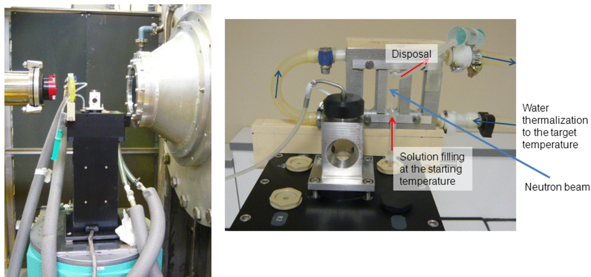
Figure S1: Photos of the modified stopped-flow cell used for time-resolved small-angle neutron scattering experiments during a temperature jump.
