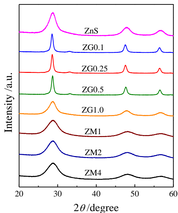
Fig. S1 XRD pattern of ZnS with different amount of graphene and MoS 2 nanosheets.
