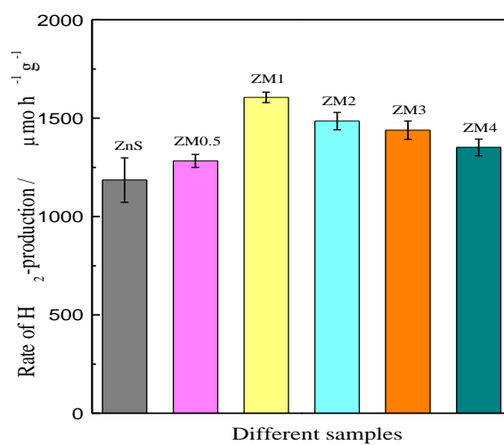
Fig.S4 H 2 production of the prepared ZnS with different amount of MoS 2
