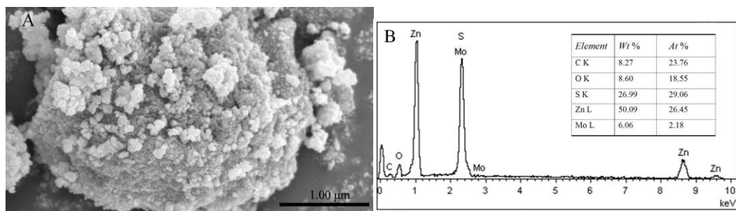
Fig.S3 SEM image (A) and EDS spectrum (B) of ZGM2.
