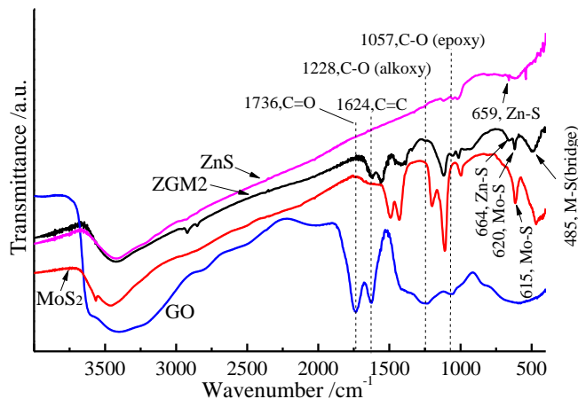
Fig. S2 FT-IR spectra of GO, ZnS, MoS 2 and ZGM2
