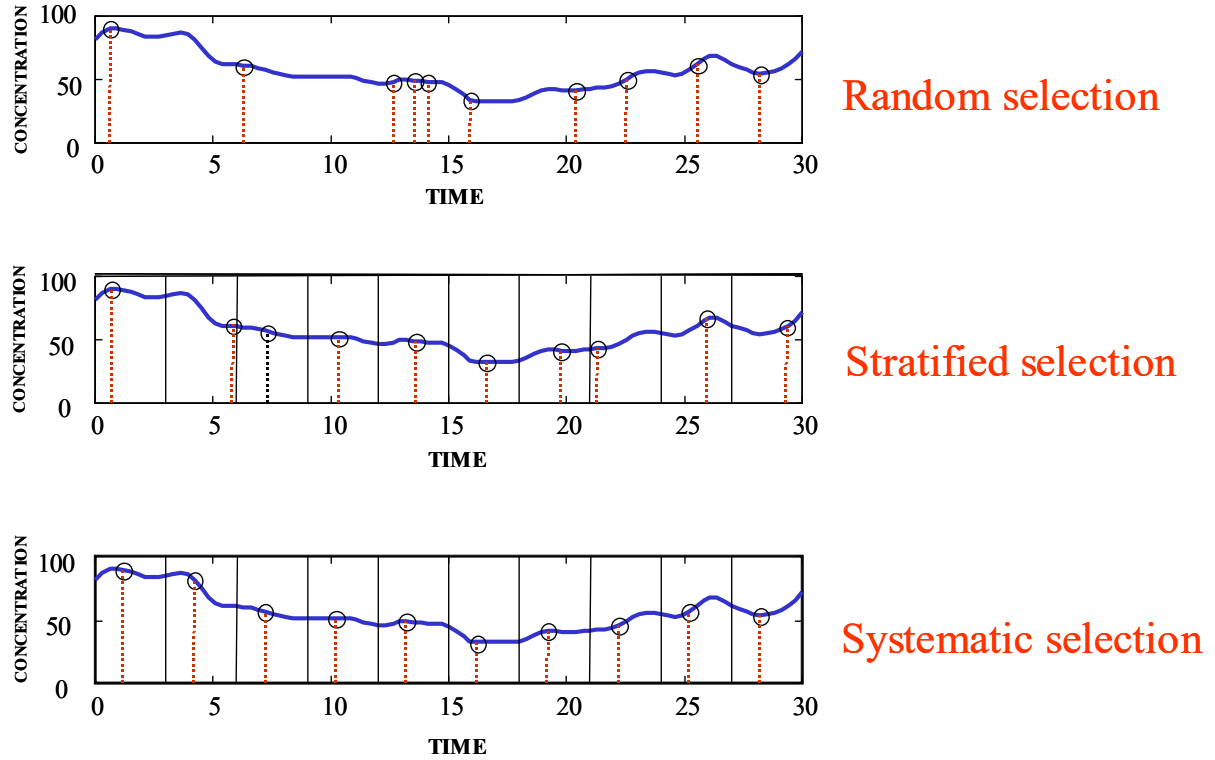
Figure C2.1: Sampling strategies
