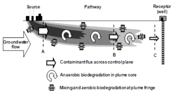
Figure 1. Conceptual model for natural attenuation of hydrocarbon compounds in groundwater.
