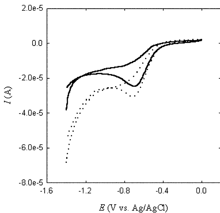
Cyclic voltammogram of electrode modified by cubic phase MO containing ZnTPP in the absence (solid line) and presence (dotted line) of 0.1 \text{ mM } \text{CCl}_4 . Scan rate = 5 \text{ mV s}^{-1} .
