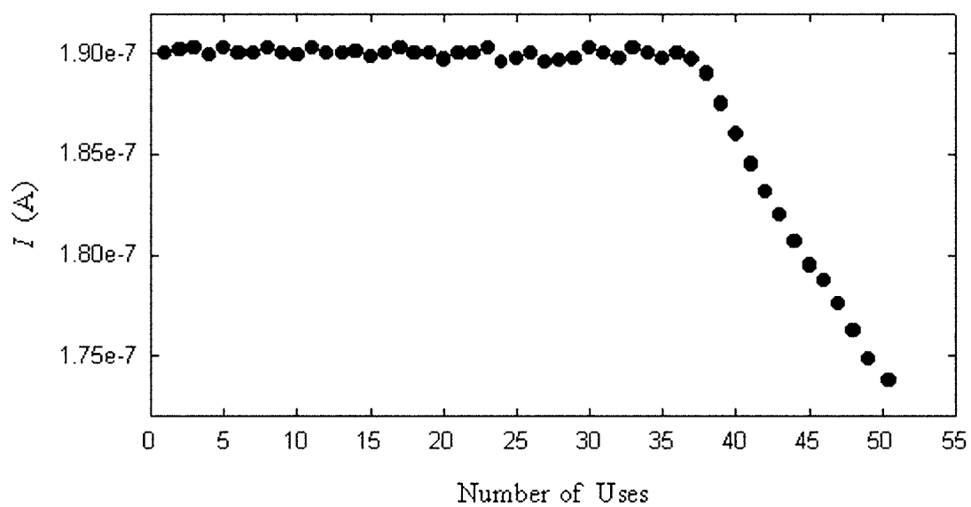
Amperometric responses at -1.0 \text{ V} to 0.4 \mu\text{M Cl}_4 at a single electrode modified by ZnTPP-containing MO cubic phase.
