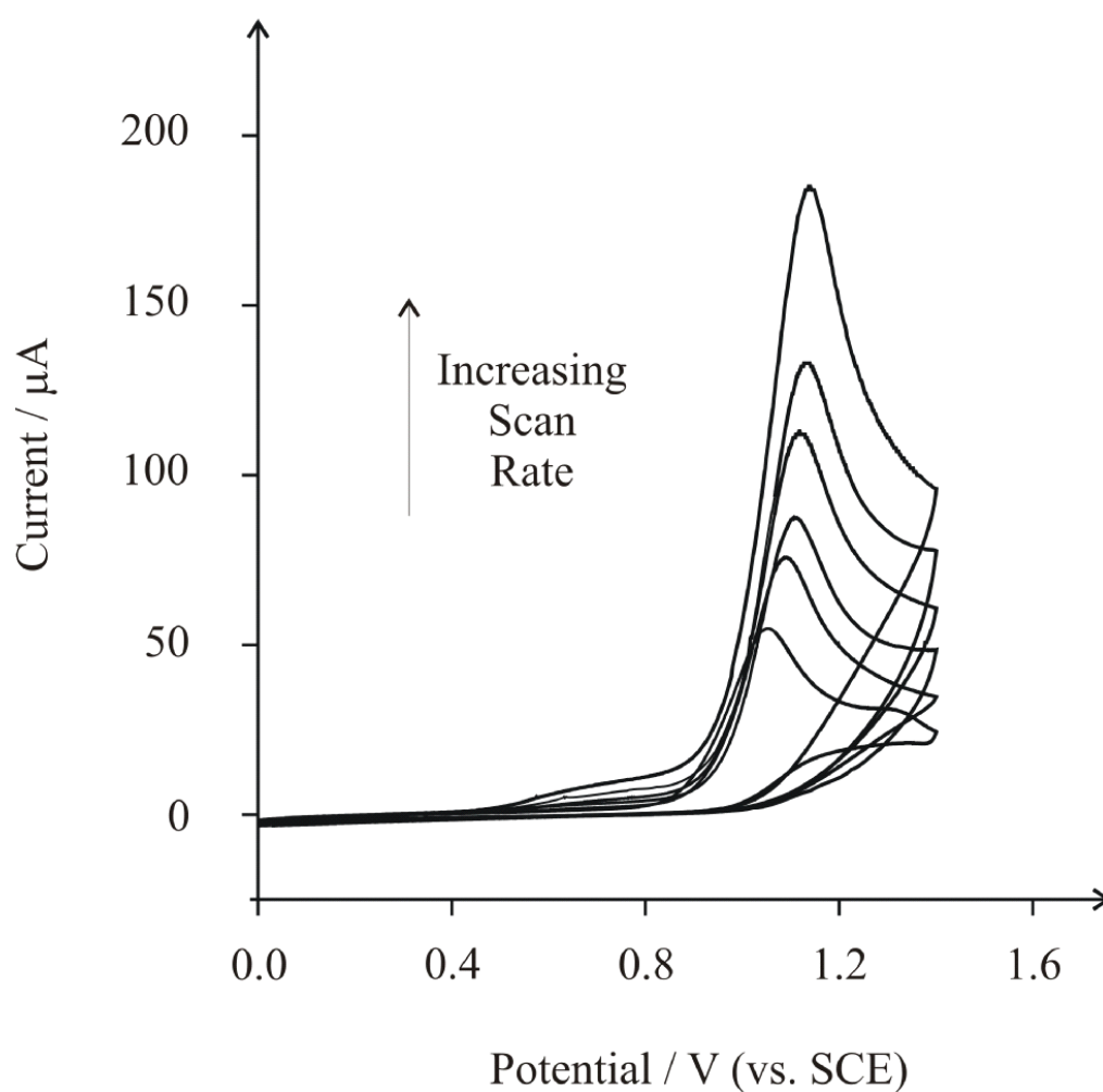
ESI A Response of increasing the scan rate at a boron-doped diamond electrode (3 mm diameter) in a 0.1 M KCl solution which has had 0.1 % ammonia bubbled through it for 30 minutes. The scan rates are (from bottom to top) 50, 100, 200, 300, 500, 800 \text{mV s}^{-1} .
