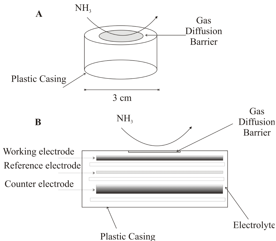
ESI B Schematic representation of an electrochemical gas sensor (A) incorporating a gas diffusion membrane which is approximately 3 cm by 1.5 cm. The sensor is based on a three-electrode arrangement (B) with BDD as the working electrode with a graphite counter and a silver wire as the reference electrode. The supporting electrolyte was 0.1 M KCl.
