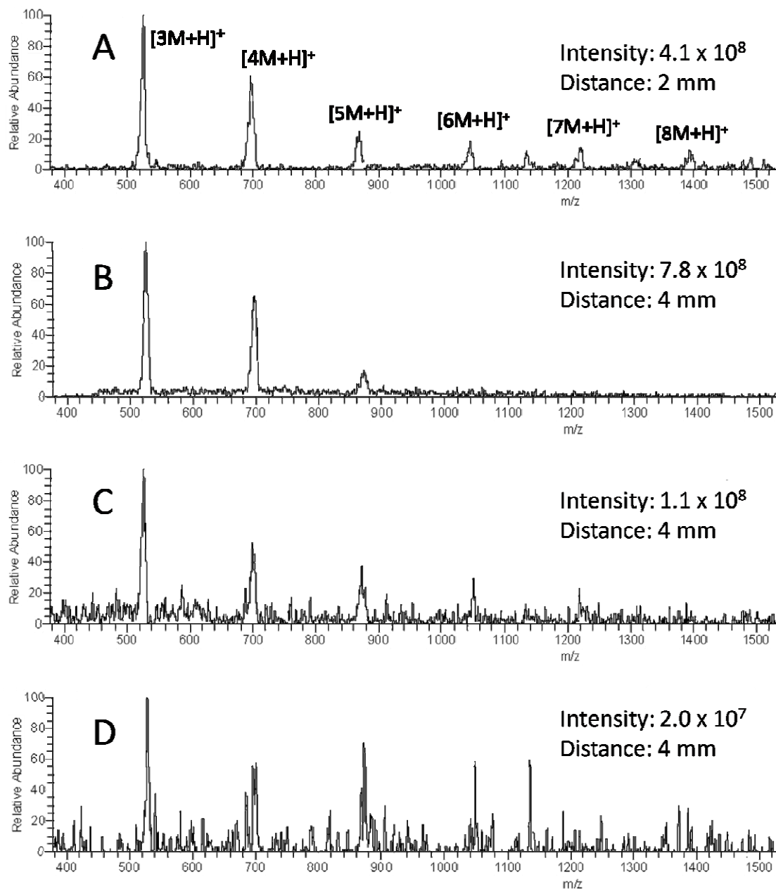
Fig. S1 The effects of varying sprayer position and orientation on the performance of the version 2 RIT array.
