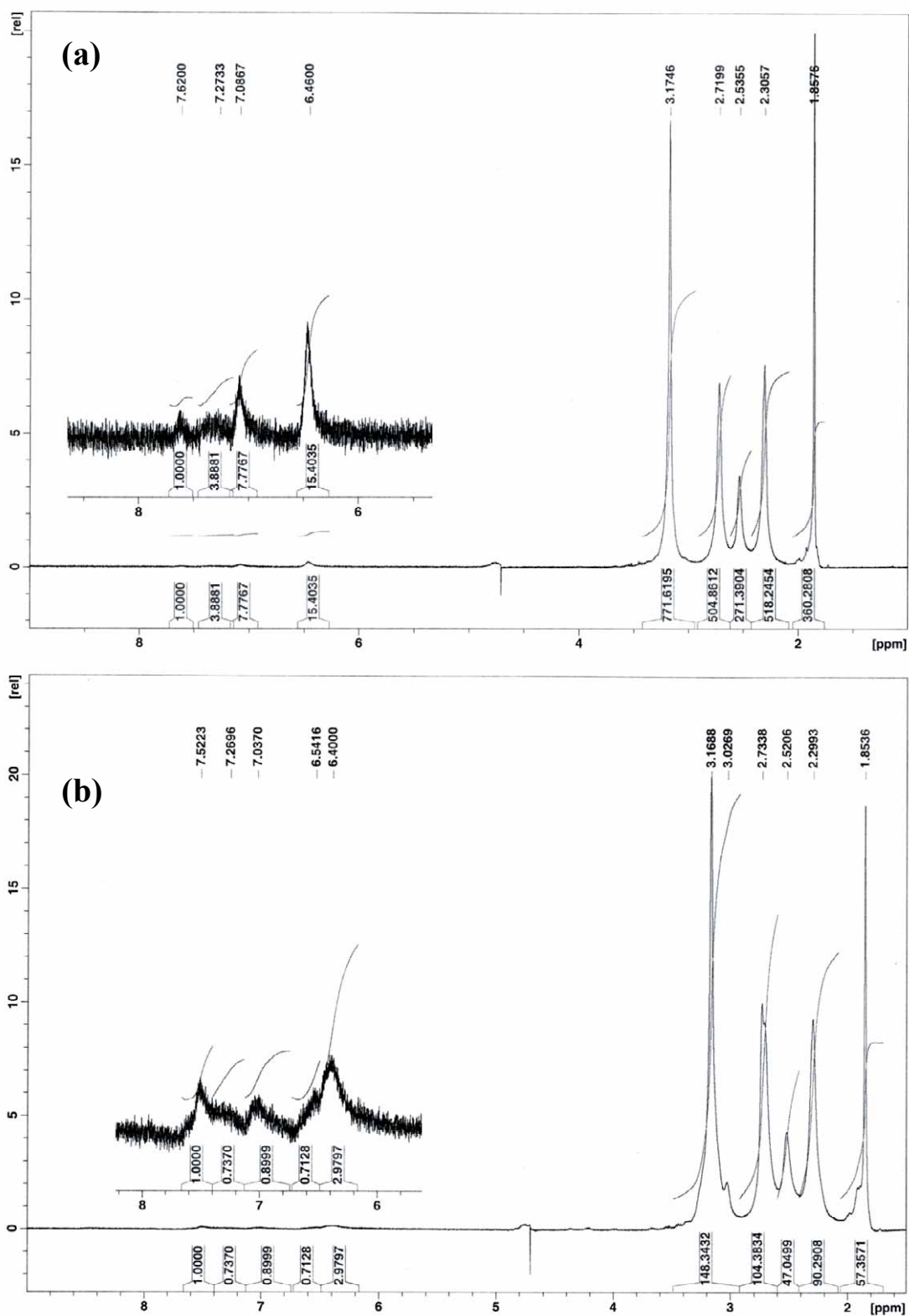
Figure S1. ^1\text{H} NMR spectra of the DSNPs \{(\text{Au}^0)_7\text{-G5.NHAc-FI}\} (a) and \{(\text{Au}^0)_7\text{-G5.NHAc-FI-FA}\} (b).
