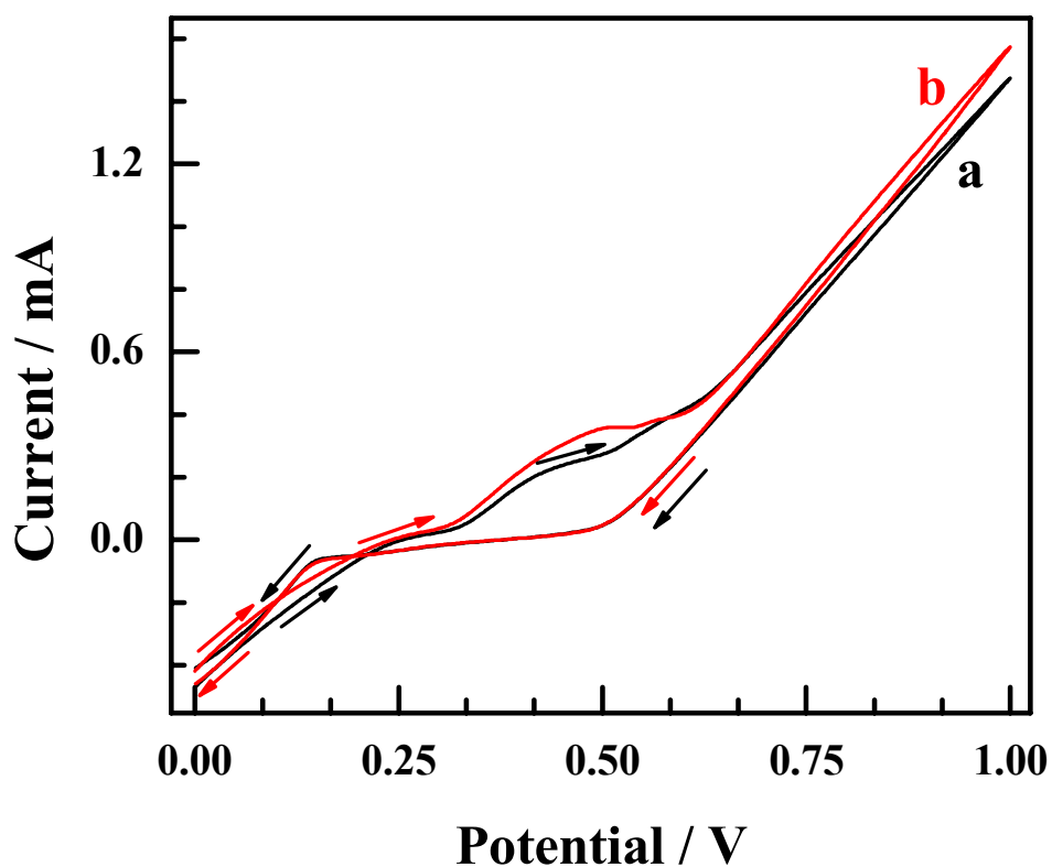
Fig. S1: CV of Ag-macro electrode in pH 7.0 phosphate buffer in the absence (a) and presence (b) of 1.0 mM NaNO 2 . Scan rate = 20 mV s -1 .
