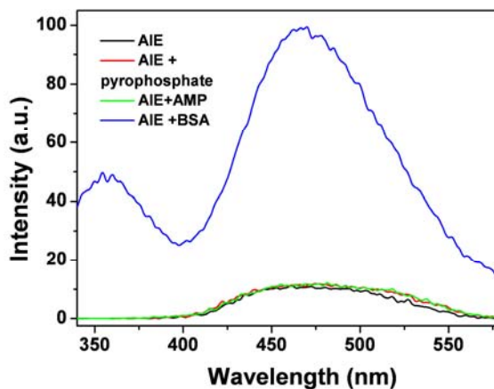
Fig S2 The influence of adenosine-5'-phosphoric acid (AMP) and pyrophosphate on the fluorescence quenching efficiency
