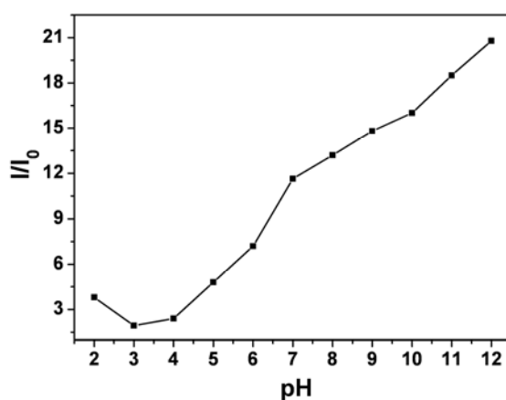
Fig S1 The effect of pH on the fluorescence enhancement of AIE probe and BSA.
