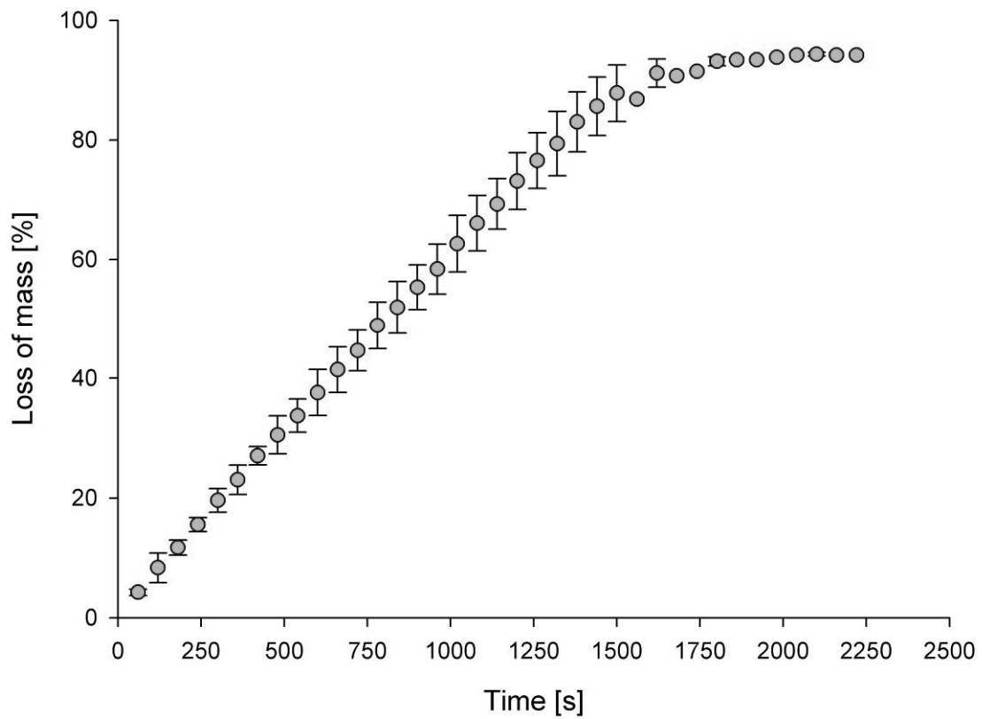
Supplementary Figure 1. Percentage loss of mass monitored over time as a result of evaporation of the normal clotting plasma sample applied to the open lateral flow channel device (n=3).
