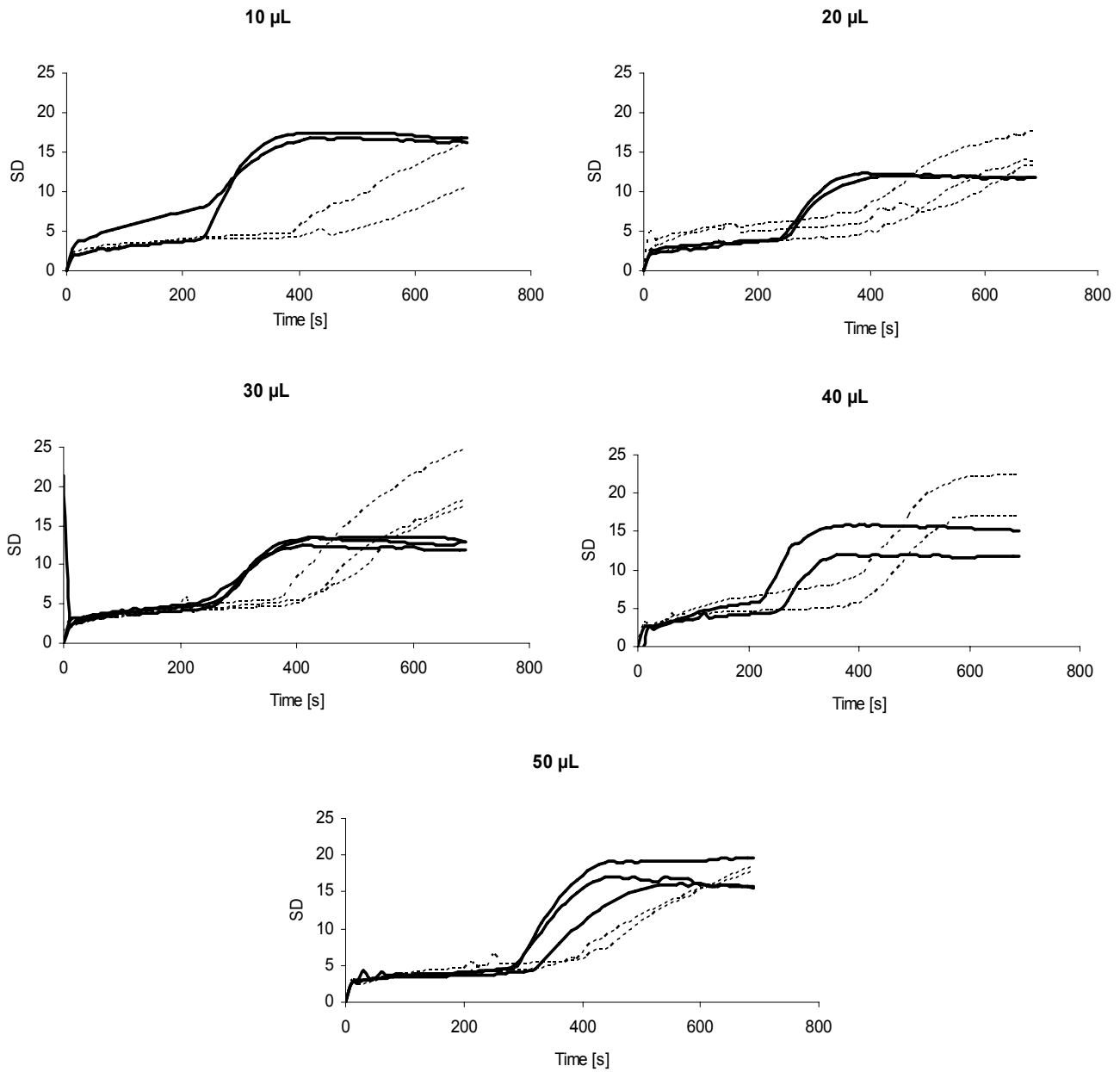
Supplementary Figure 2. Change in SD over time obtained for plasma spiked with 0 (solid line) and 0.5 U/mL of heparin (dotted line) tested in platforms where 10 – 50 μL of aPTT-SP were deposited and dried.
