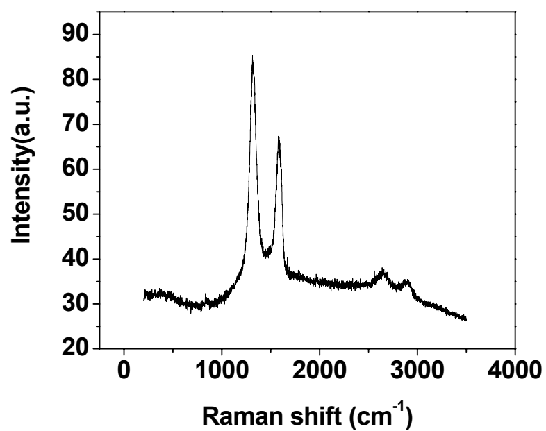
Fig.S2. Raman spectrum of graphene nanosheets.
