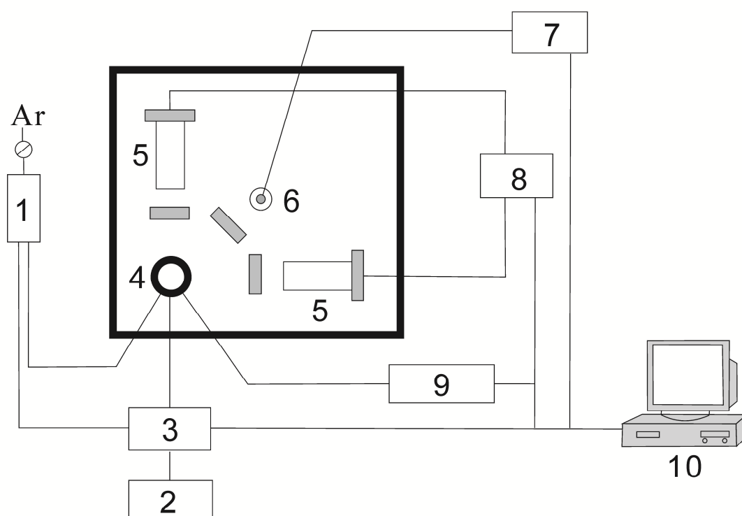
Fig. S1 Schematic diagram of the AFS-9130. (1. carrier gas supply, 2 DBD power supply, 3. DBD-PIV system, 4. atomizer, 5. hollow cathode lamp, 6. photomultiplier, 7. photomultiplier voltage, 8. lamp power supply, 9. furnace temperature controller, 10. computer)
