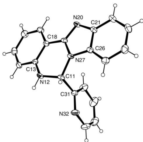
Fig. s1. ORTEP view of HL with ellipsoids at 25% probability having the numbering scheme.
