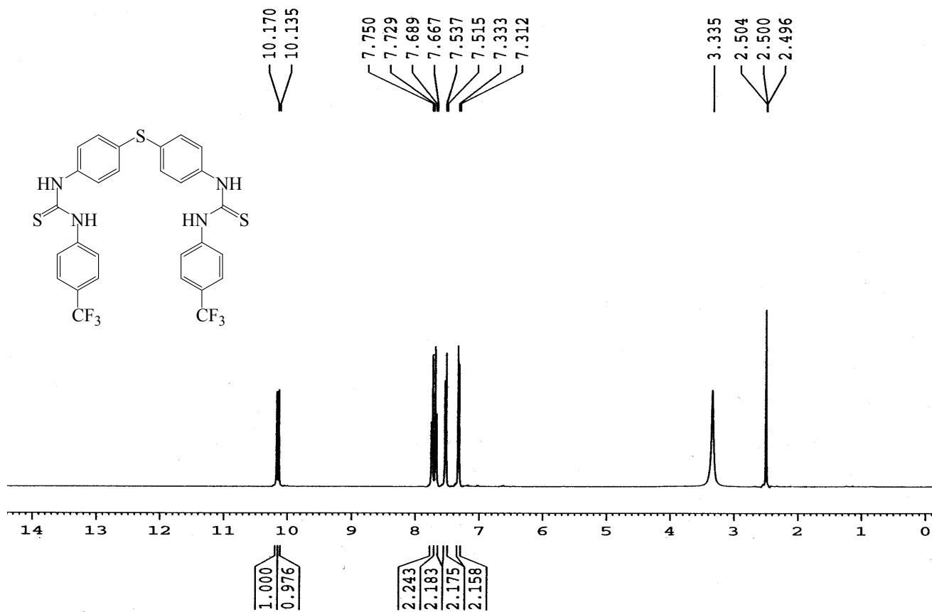
Figure S1: ^1\text{H} NMR spectrum of 1 (DMSO- d_6 )
