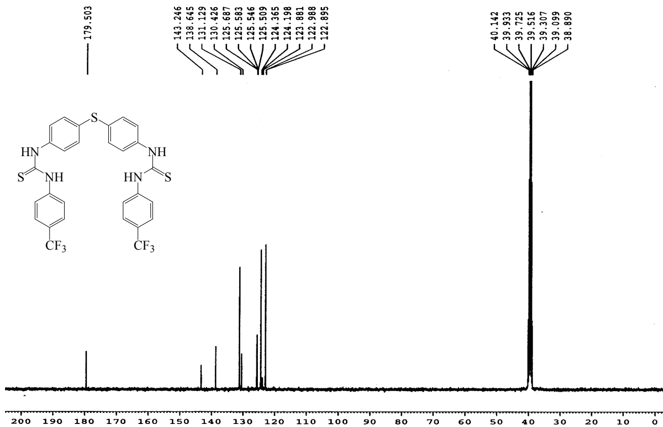
Figure S2: ^{13}\text{C} NMR spectrum of 1 (DMSO- d_6 )
