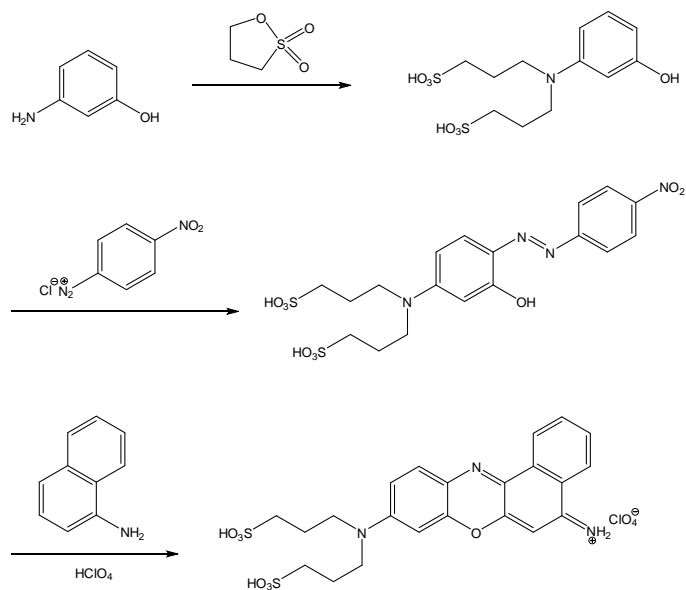
Scheme 1. Synthesis of 2SBPO dye.
