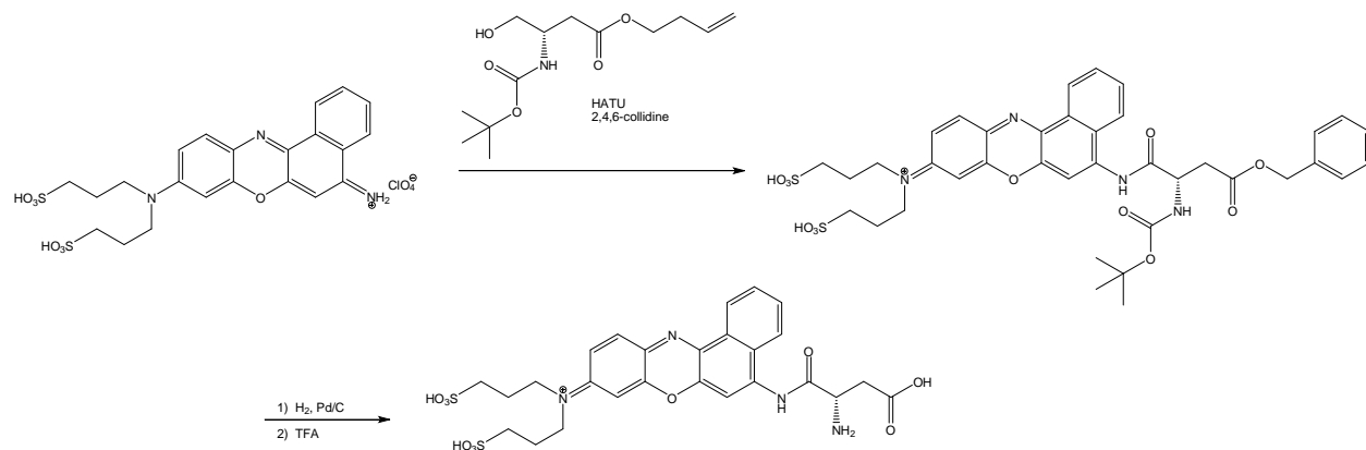
Scheme 2. Synthesis of 2SBPO-Casp
