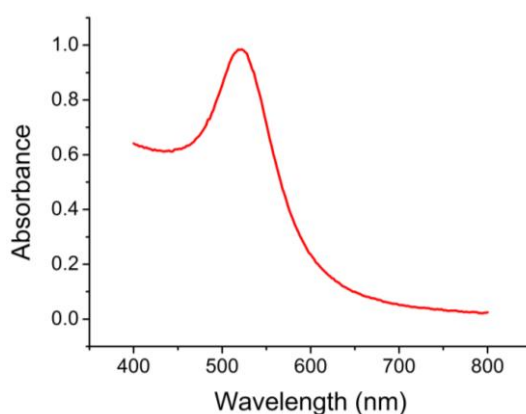
Fig. S2 Absorption spectra of 13 nm Au NP sensor solution in the presence of 6 \mu M MUA and 100 \mu M \text{H}_2\text{O}_2 .
