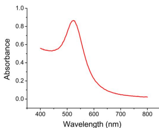
Fig. S1 Absorption spectra of the buffered Au NP solution after sequential addition of MUA (10 \mu M) and hypochlorite (30 \mu M).
