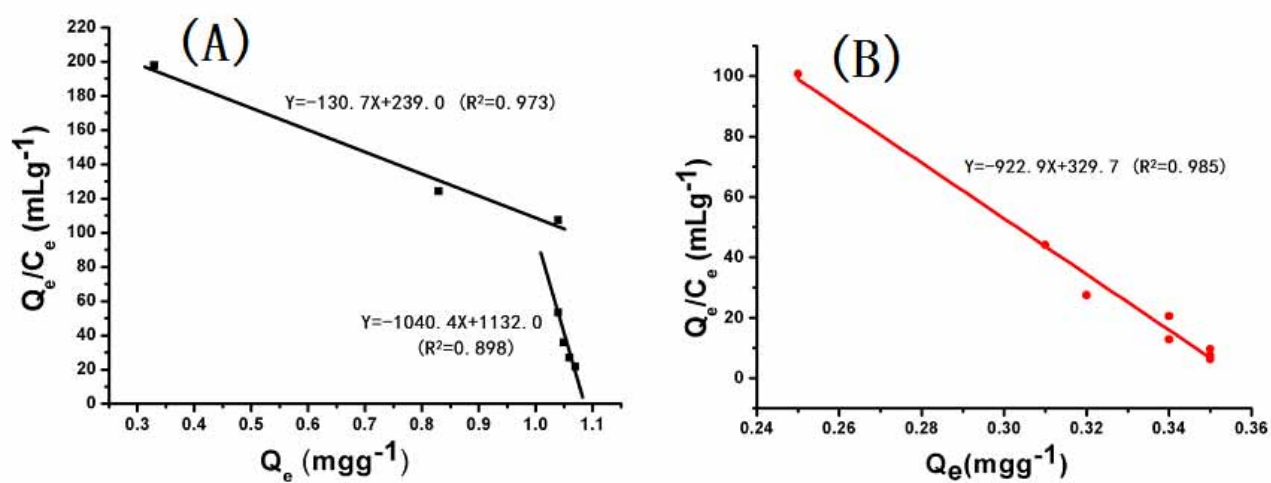
Fig. S2 Scatchard plots of MMIPs (A) and MNIPs (B).
