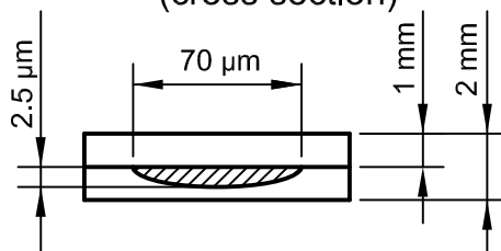
Separation channel dimensions (cross section)
