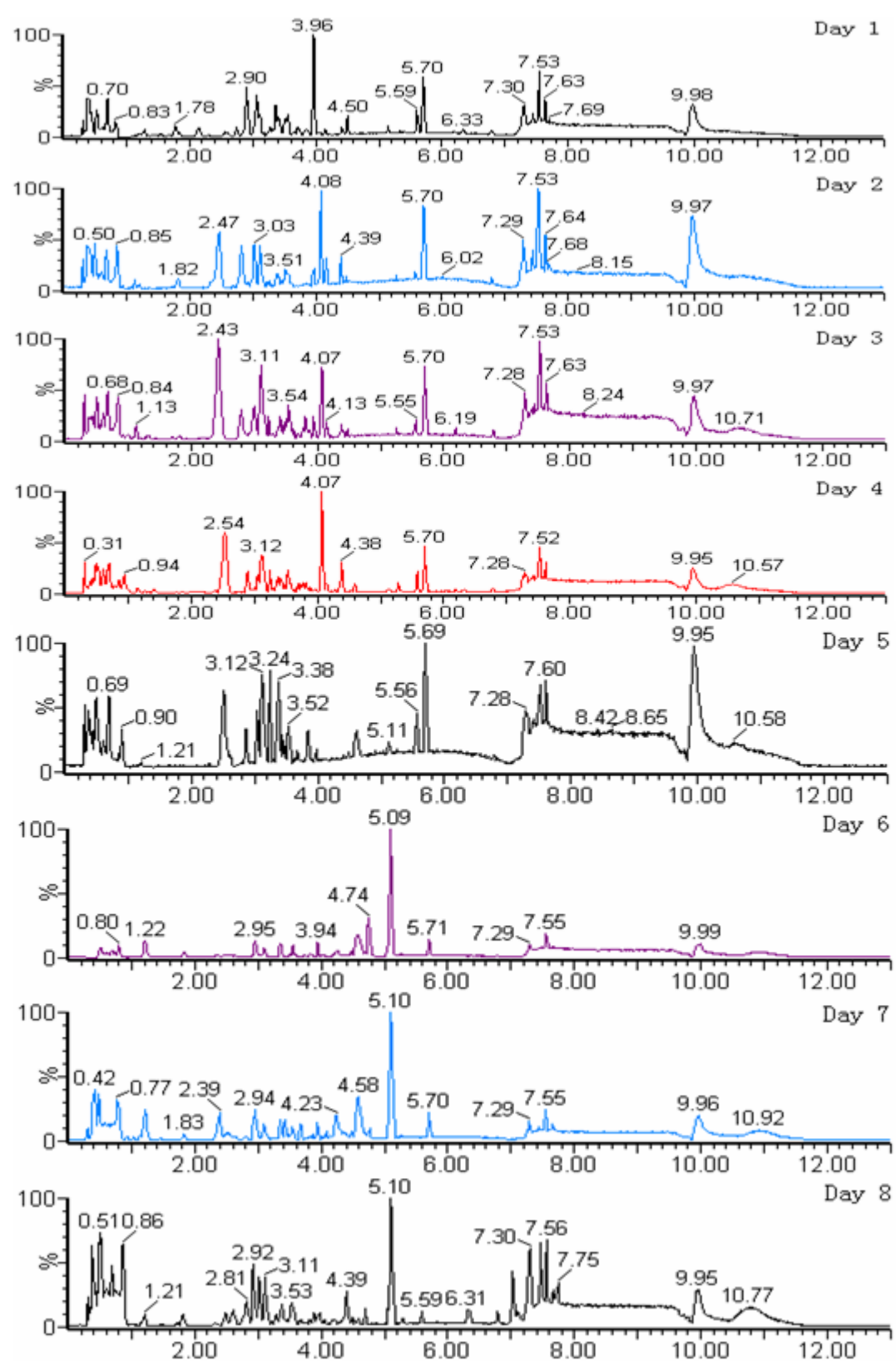
Fig.2. BPI chromatograms of urine obtain from UPLC/ESI-Q-TOF/MS analysis for continuous eight days.
