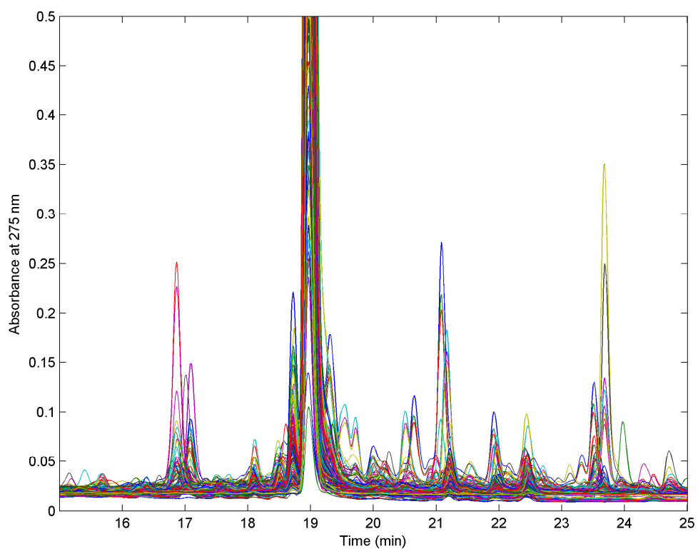
Fig. S1. Raw HPLC-DAD chromatograms for the 72 Dactylopius cochineal samples of the reference database (note that these are raw chromatograms therefore baseline was not removed and peaks were not aligned).
