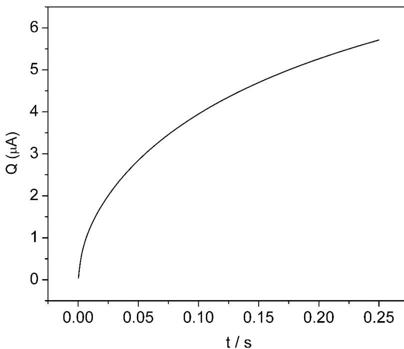
Fig S1. Plot of Q-t curve of 0.1 mM 4-NP at PMB/GCE after background subtraction.
