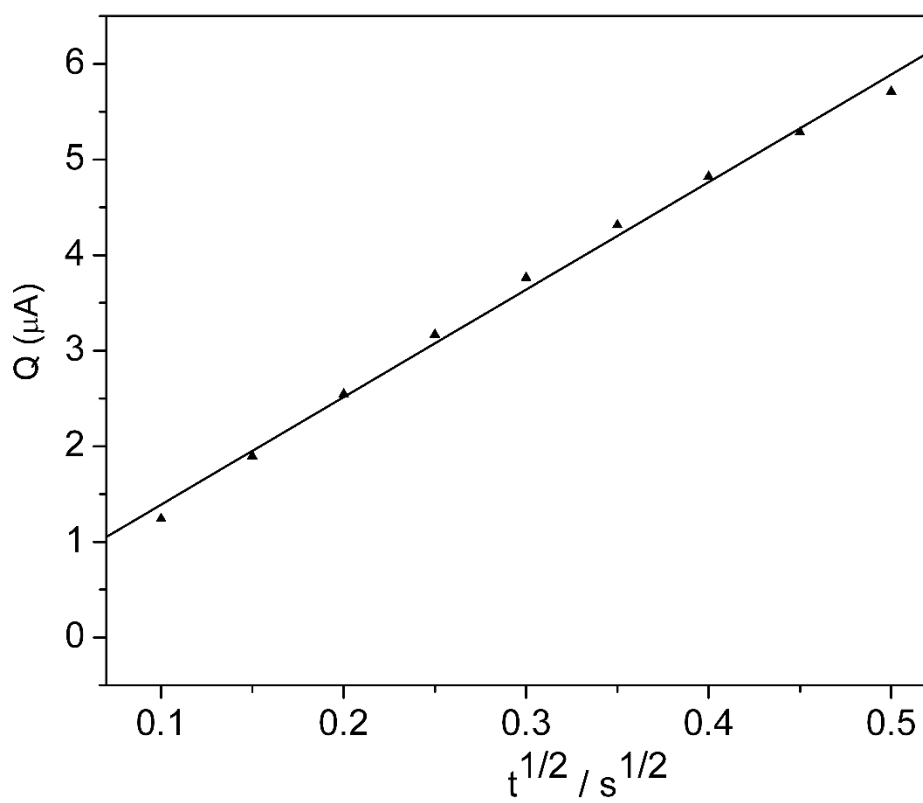
Fig S2. Plot of Q vs t^{1/2} curve.
