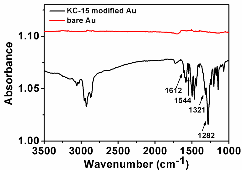
Fig S2. FTIR spectra of bare Au and KC-15 modified Au surface.
