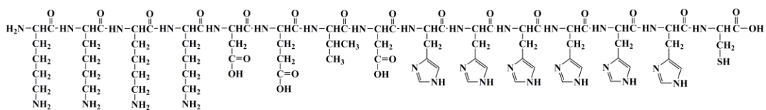
Fig S1. Chemical structure of KC-15 peptide
