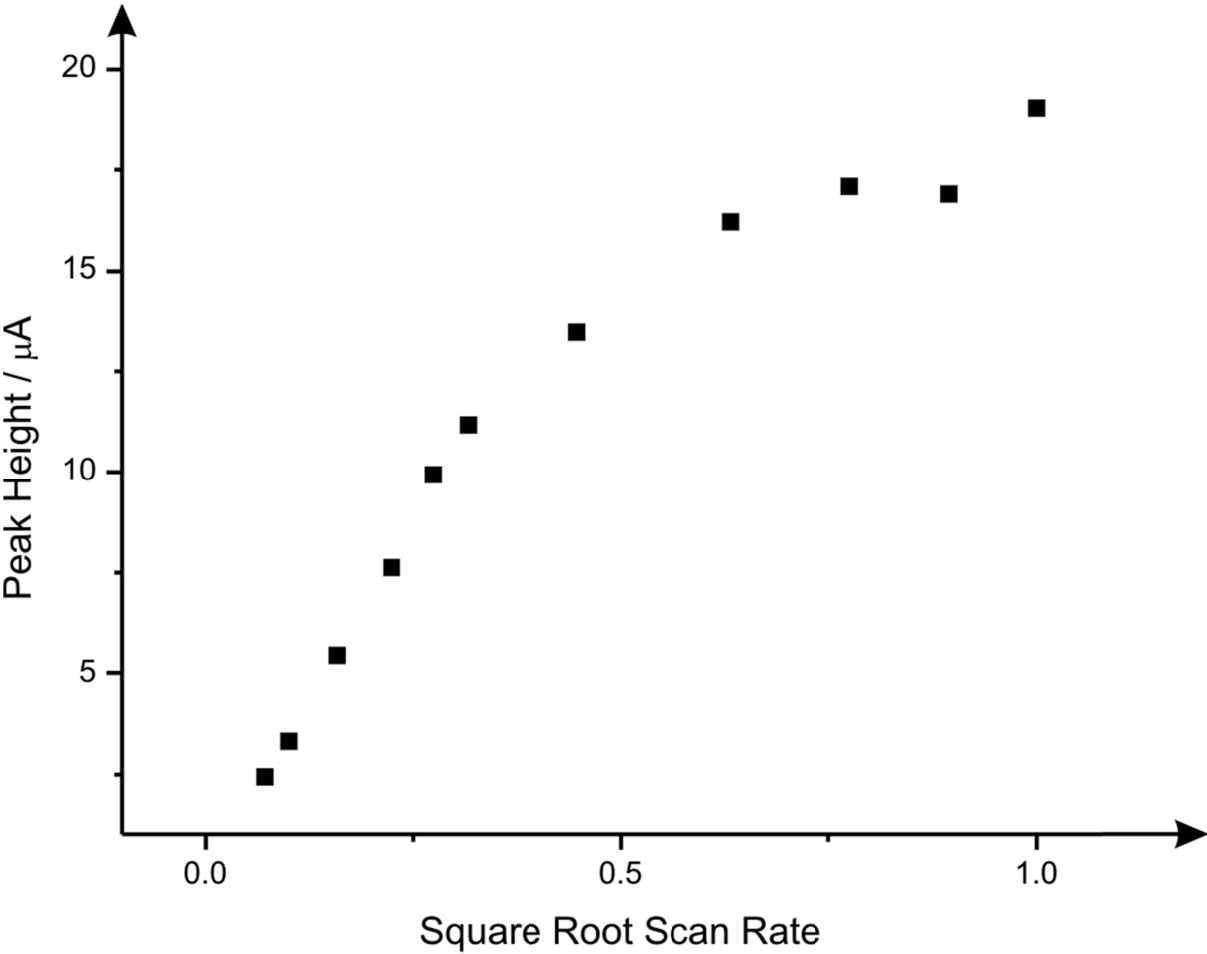
ESI 1 - A plot of peak height against the square-root of scan rate for 3a .
