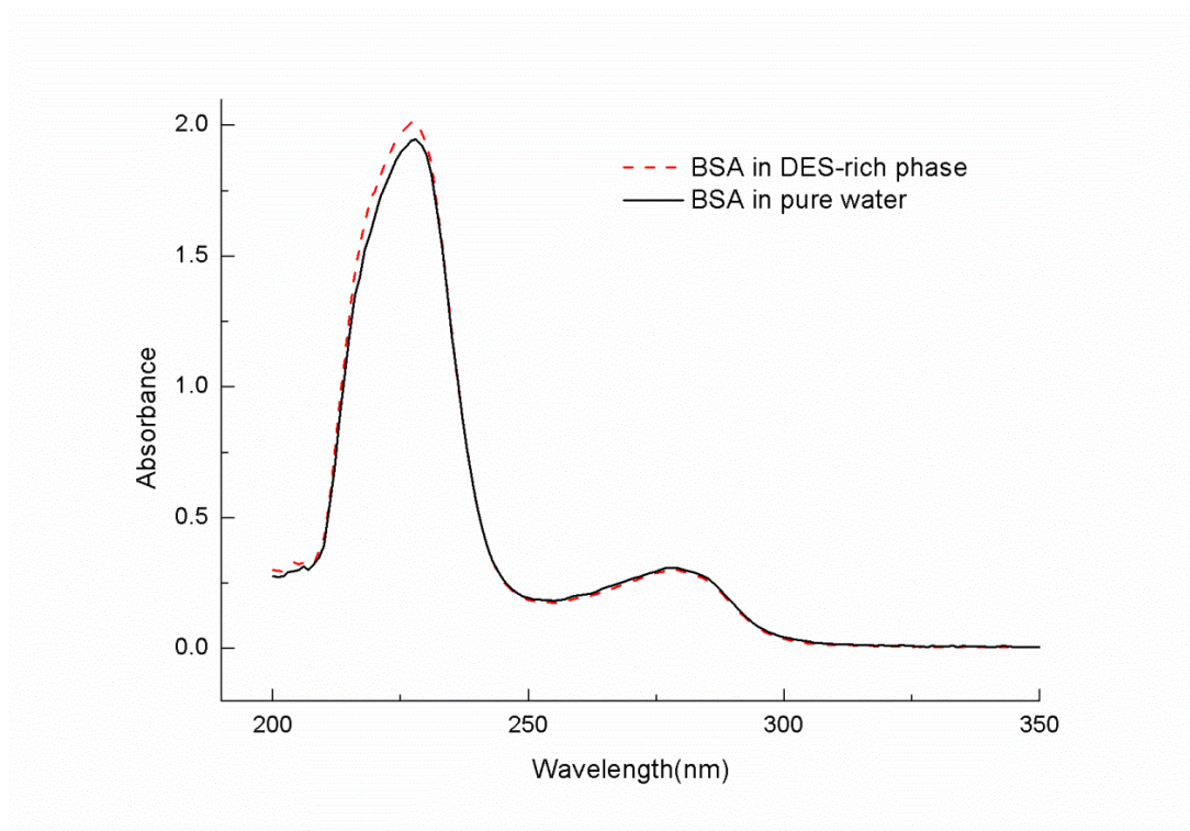
Figure S3. UV-vis spectra of BSA in pure water and in DES-rich top phase after extraction.
