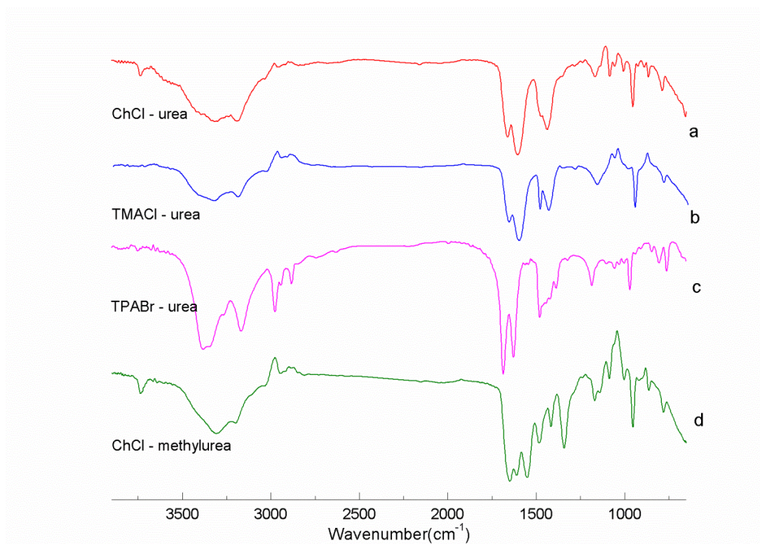
Figure S1. The FT-IR spectra of the four deep eutectic solvents.
