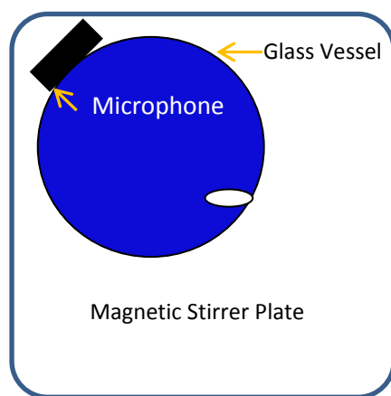
Figure 1: Schematic diagram of BARDS spectrometer
