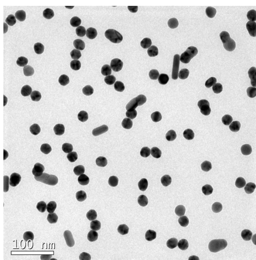
Fig.S1: Low magnification TEM image of 1:2 ratio HAuCl 4 :Ascorbic acid
