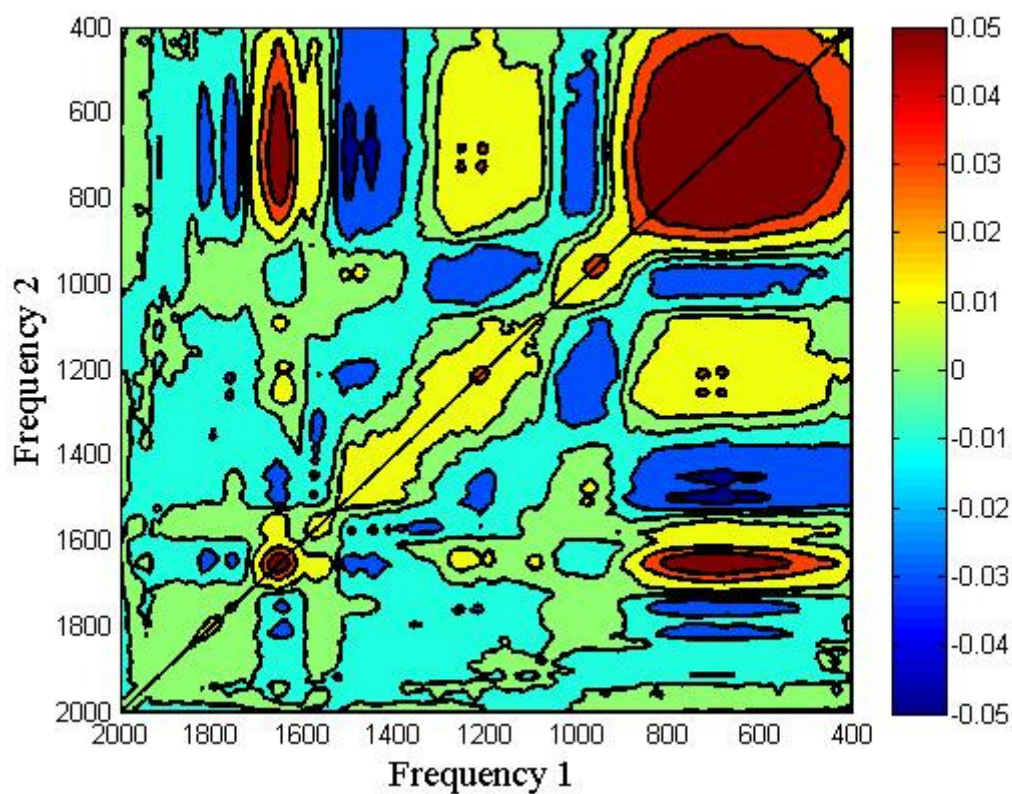
2D Synchronous correlation map (Fig 9A)
