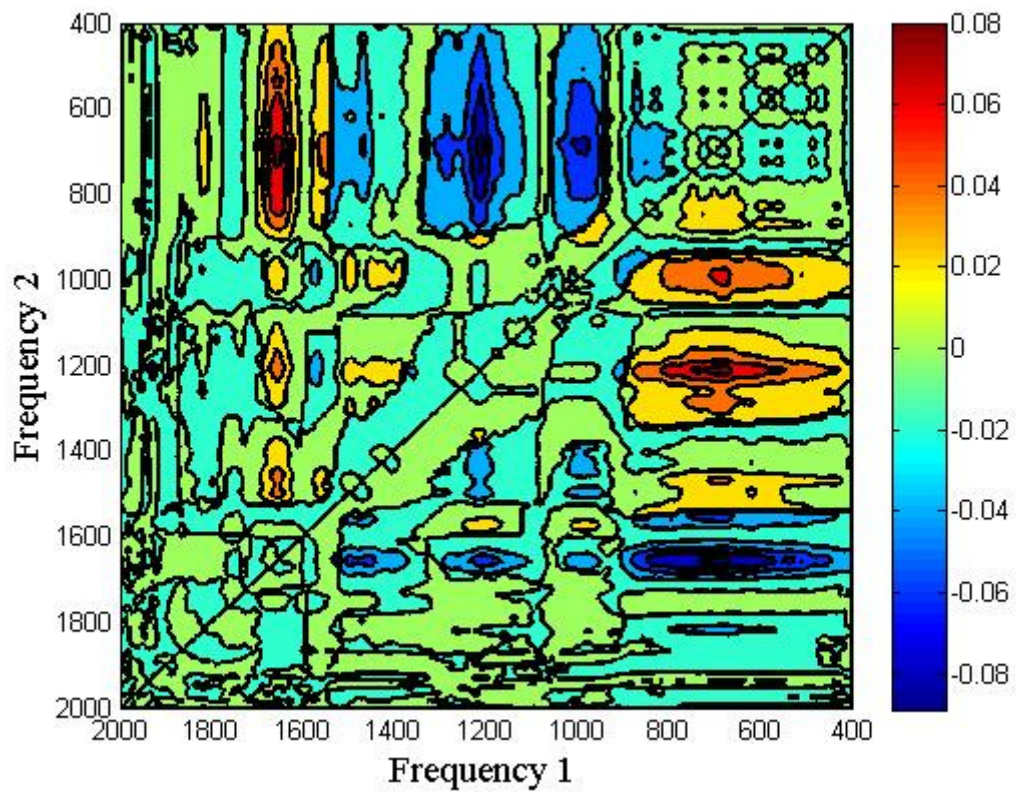
2D Asynchronous correlation map (Fig 9B)
