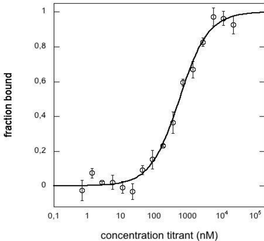
Figure S1: MST assay for ampicillin binding Ampicillin284 with a K_d of 569.8 \pm 76.2 nM and an R^2 of 0.990.
