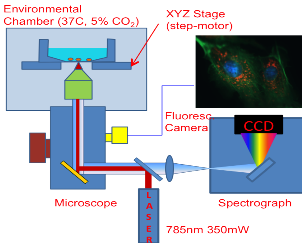
Figure S1: Schematic description of the Raman micro-spectrometer for molecular analysis of live cells.
