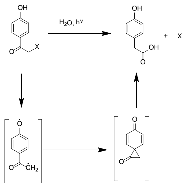
Scheme 1. The mechanism for the Favorskii reaction
