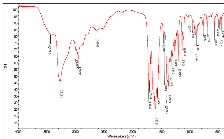
Supplementary figure 4: IR spectrum of dicycloplatin
