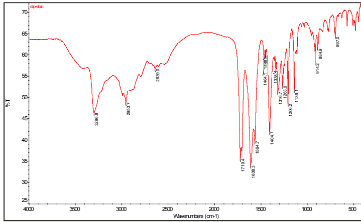
Supplementary figure 6: IR spectrum of physical abrasive mixtures of carboplatin and cyclobutane dicarboxylate powder
