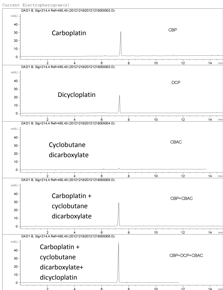
Supplementary figure 1: Separation of carboplatin and dicycloplatin by aqueous capillary electrophoresis
