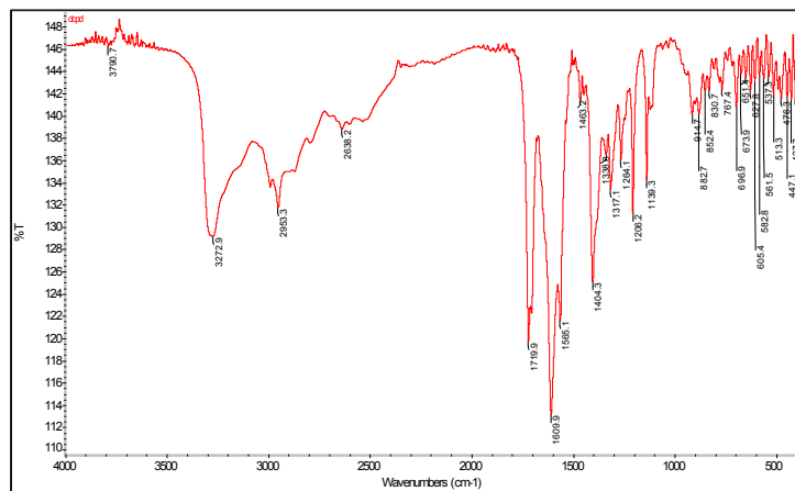
Supplementary figure 5: IR spectrum of lyophilized (mixture) powders of carboplatin and cyclobutane dicarboxylate
