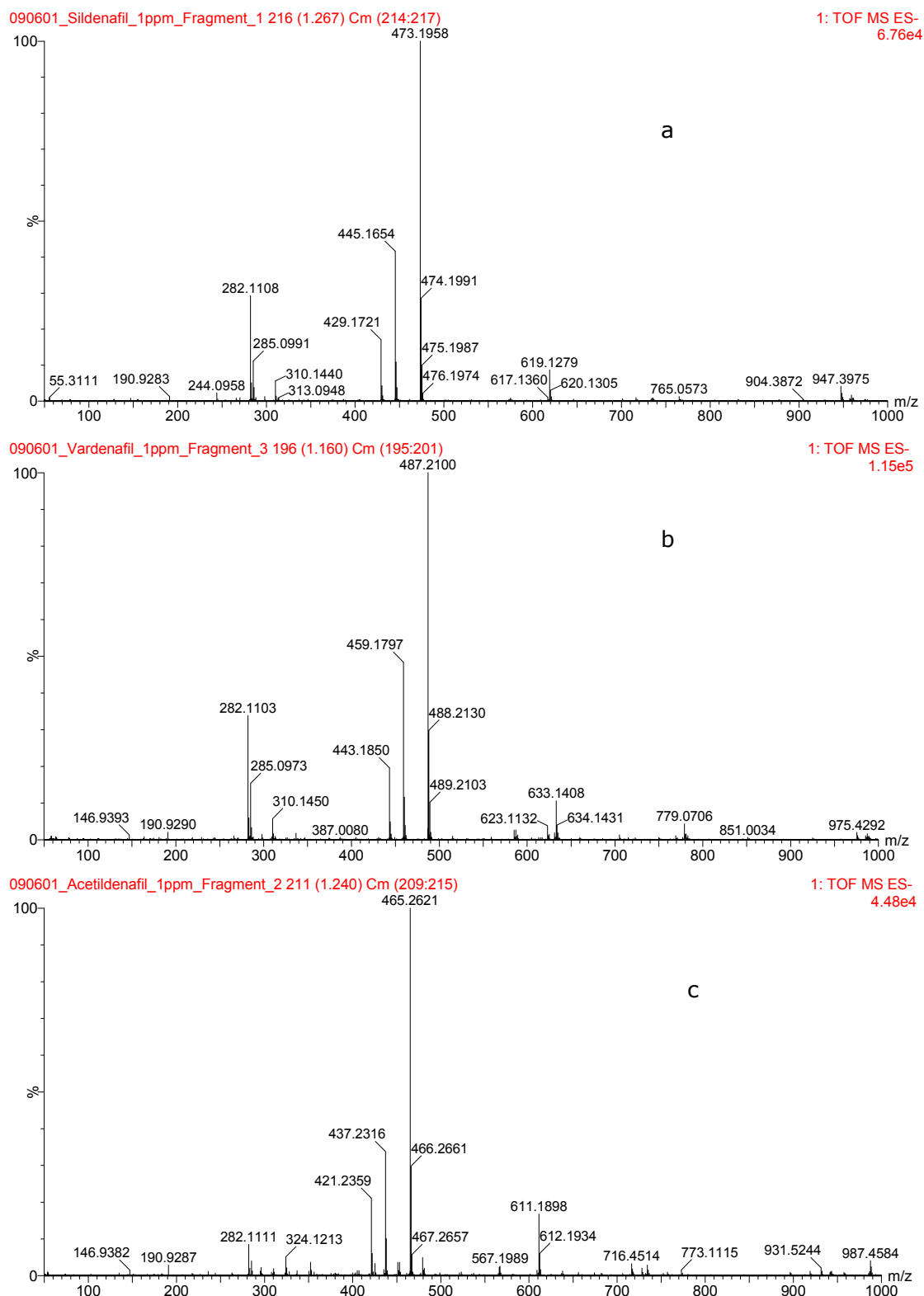
Figure S3. In-source CID spectra of (a) Sildenafil, (b) Vardenafil and (c) Acetildenafil under ESI –ve mode in TOF.
