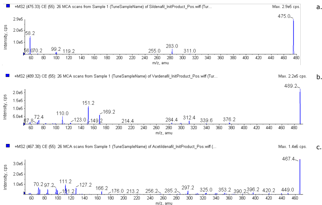
Figure S1. MS 2 spectra of (a) Sildenafil, (b) Vardenafil and (c) Acetildenafil in +ve mode
