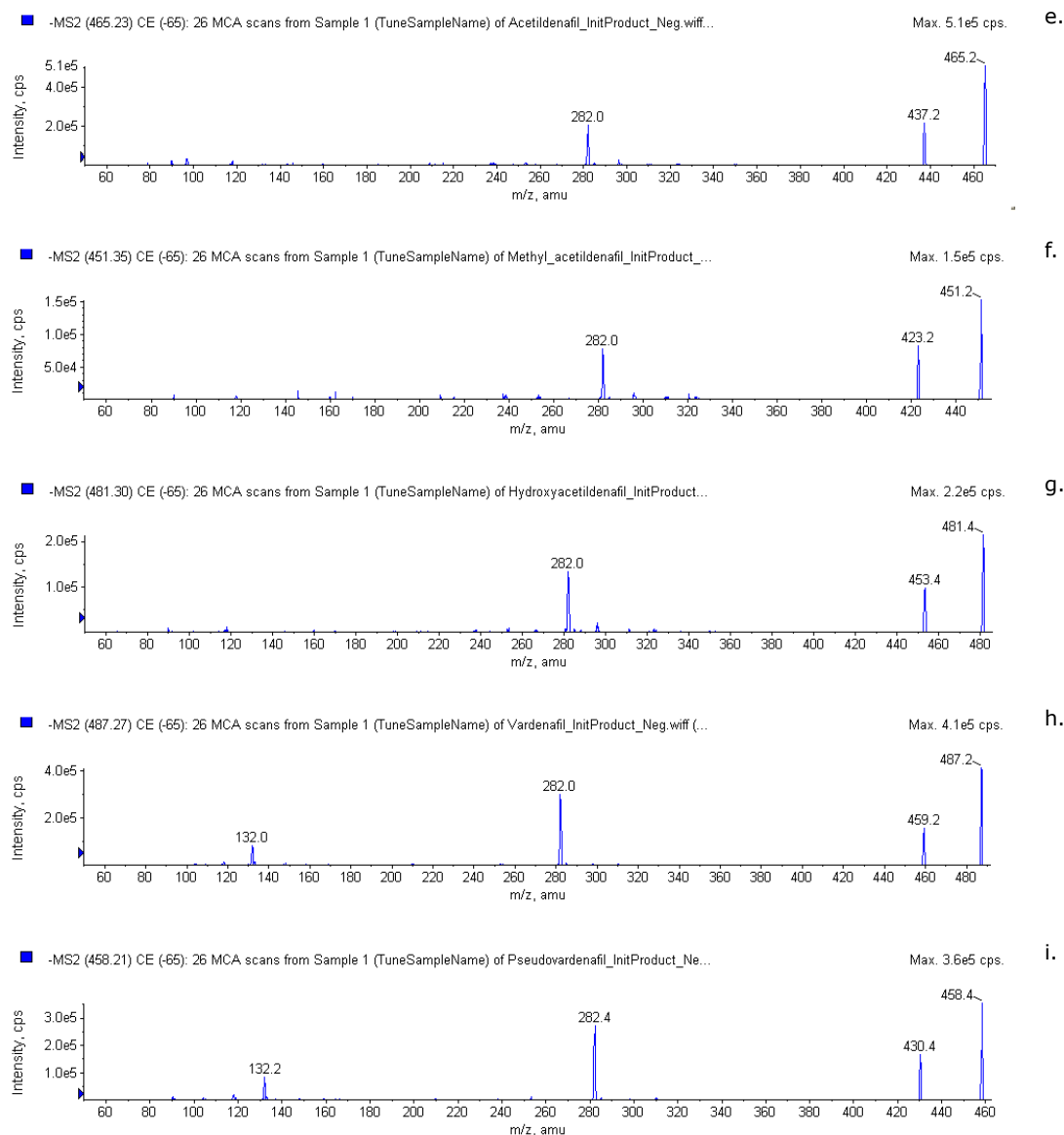
Figure S2. MS 2 spectra of (a) Sildenafil, (b) Homosildenafil, (c) Hydroxyhomosildenafil, (d) Piperidino sildenafil, (e) Acetildenafil, (f) noracetildenafil, (g) Hydroxyacetildenafil, (h) Vardenafil and (i) Piperidino vardenafil in -ve mode
