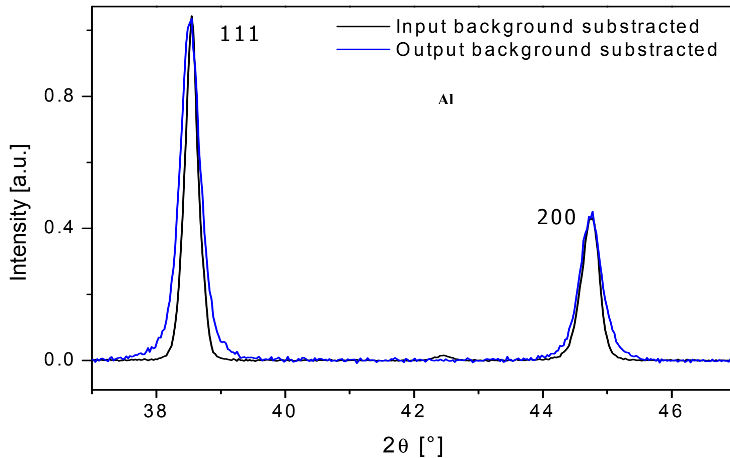
Fig. 3. XRD confirming the decrease in particle size of Al after milling with 10% C w/w for 1hr in Retsch ball mill.
