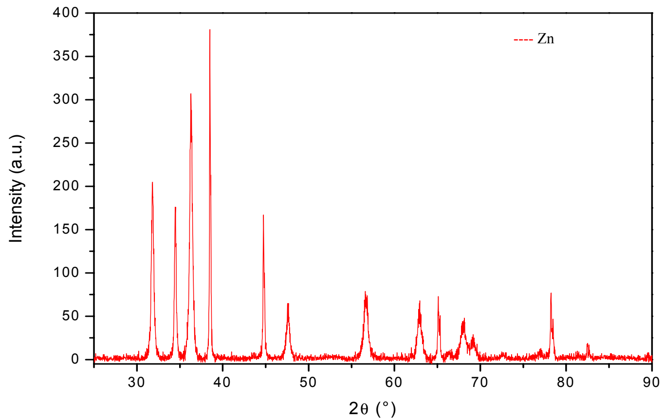
Fig. 1. XRD confirming the presence of Zn in the 1hr Retsch ball milled ZnO and Al mixture
